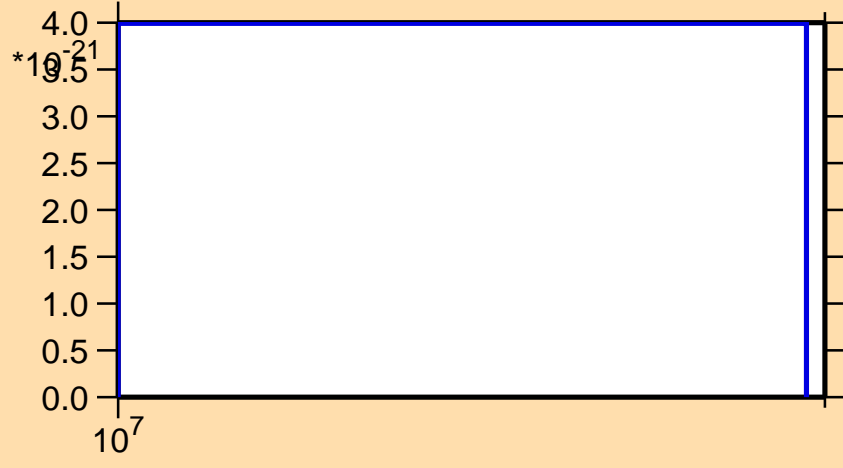
\sigma vs. E for ^{242}\text{Cf} (mt 42)
