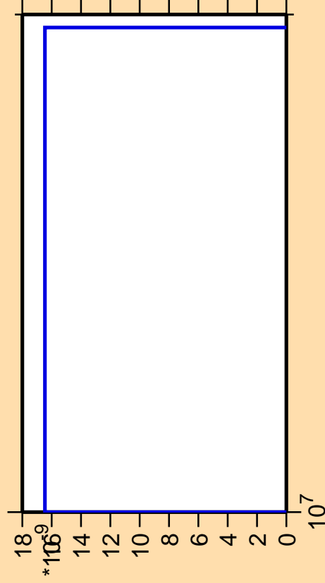
\Delta\sigma/\sigma vs. E for ^{242}\text{Cf} (mt 42)
