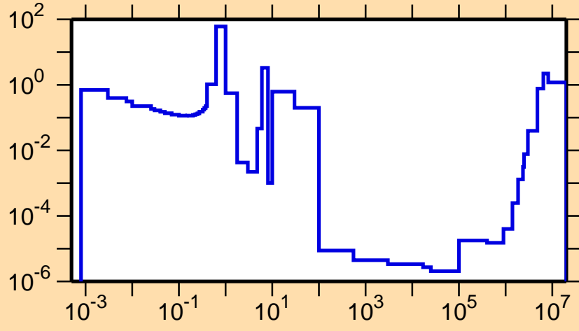
\sigma vs. E for ^{242}\text{Cf}(n,f)
