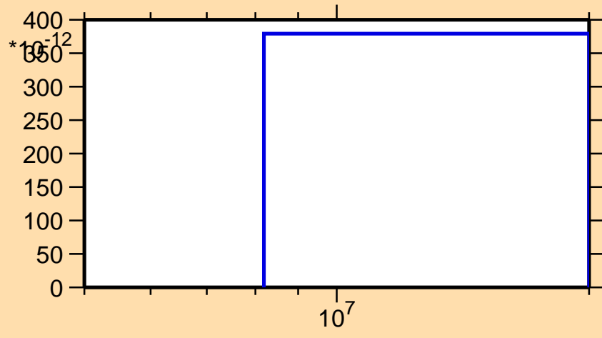
\sigma vs. E for ^{242}\text{Cf}(n,\text{He3})
