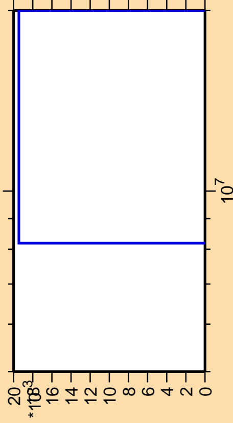
\Delta\sigma/\sigma vs. E for ^{242}\text{Cf}(n,3n\alpha)
