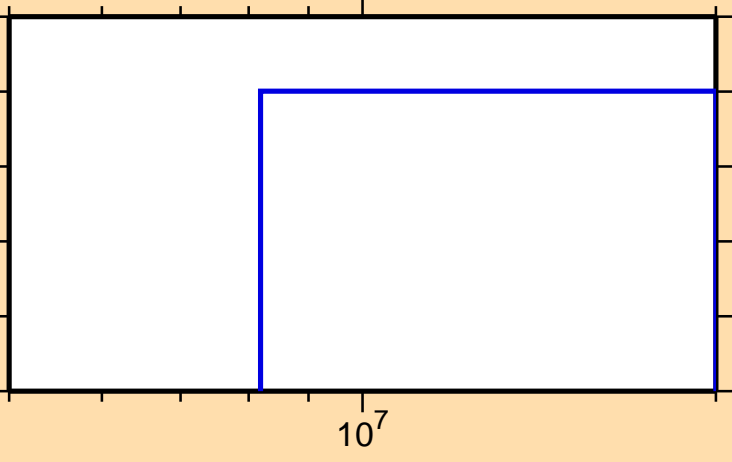
\sigma vs. E for ^{242}\text{Cf}(n,3n)
