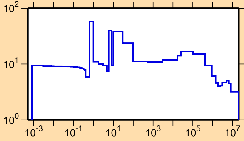
\sigma vs. E for ^{242}\text{Cf}(n,\text{el.})
