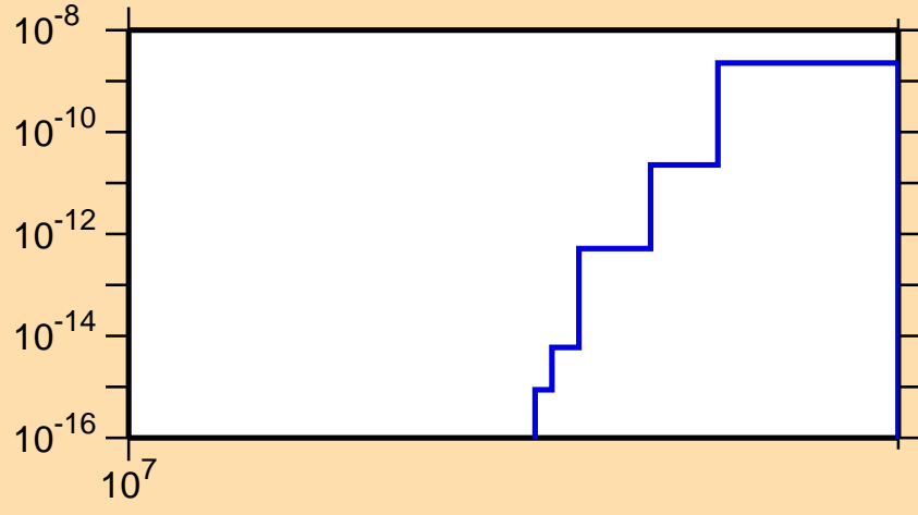
\sigma vs. E for ^{243}\text{Cf}(n,nt)
