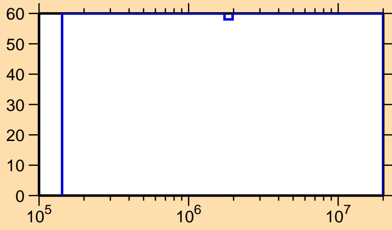
\Delta\sigma/\sigma vs. E for ^{243}\text{Cf}(n,n_1)
