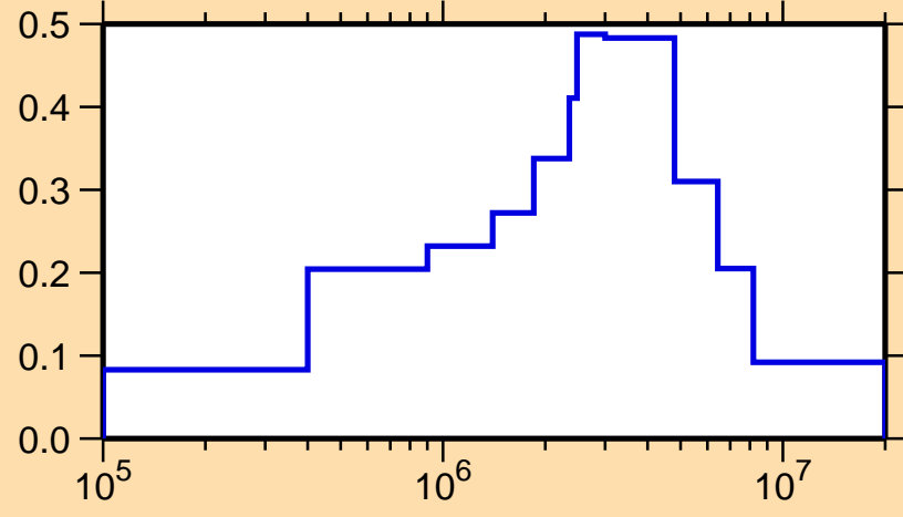
\sigma vs. E for ^{243}\text{Cf}(n,n_1)
