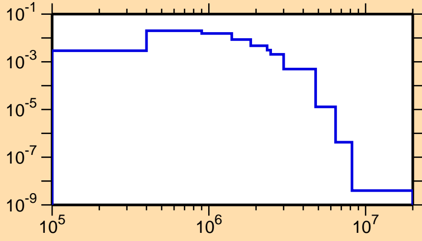
\sigma vs. E for ^{243}\text{Cf}(n,n_3)
