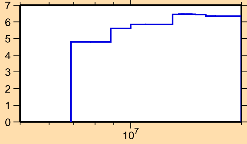
\Delta\sigma/\sigma vs. E for ^{244}\text{Cf}(n,\text{nonel.})
