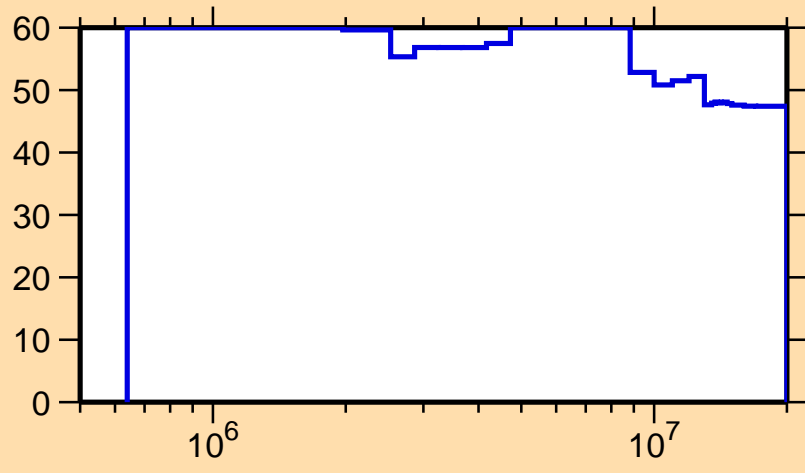
\Delta\sigma/\sigma vs. E for ^{244}\text{Cf}(n,n\text{cont.})
