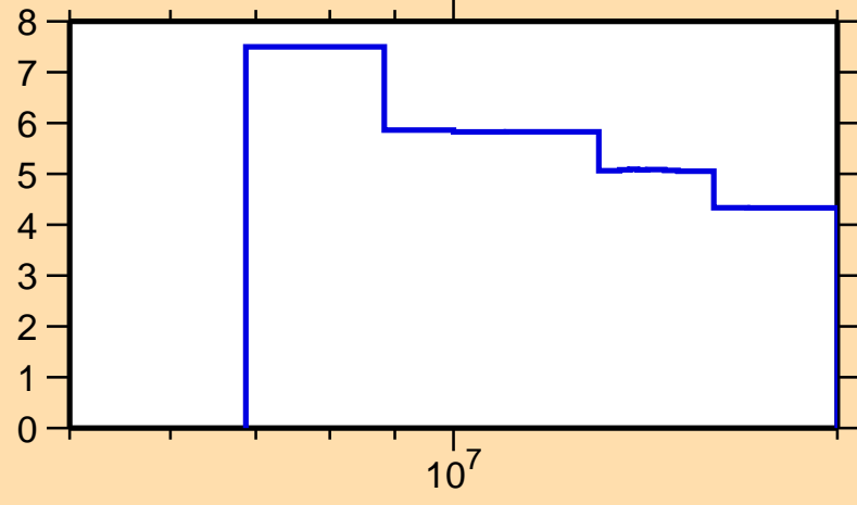
\Delta\sigma/\sigma vs. E for ^{244}\text{Cf}(n,\text{tot.})
