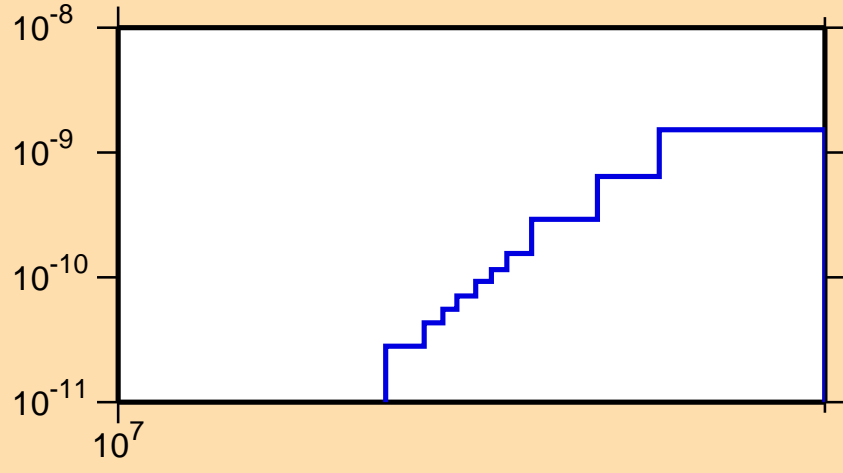
\sigma vs. E for ^{244}\text{Cf}(n,p\alpha)
