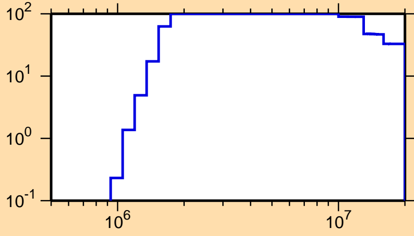
\Delta\sigma/\sigma vs. E for ^{244}\text{Cf}(n,p)
