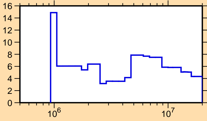
\Delta\sigma/\sigma vs. E for ^{244}\text{Cf}(n,\text{tot.})
