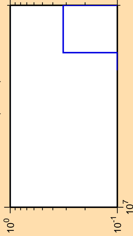
\Delta\sigma/\sigma vs. E for ^{244}\text{Cf}(\text{mt } 34)
