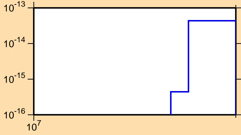
\sigma vs. E for ^{244}\text{Cf}(\text{mt } 34)
