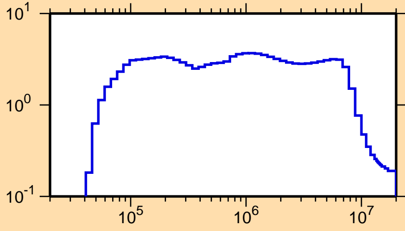
\sigma vs. E for ^{244}\text{Cf}(n,\text{inel.})
