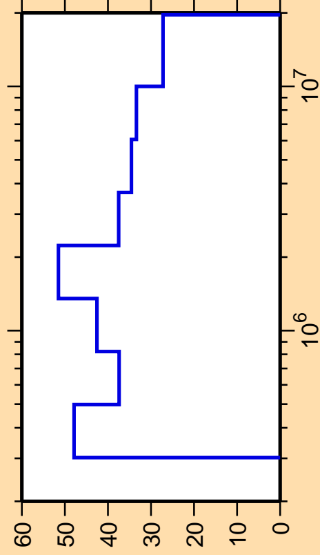
\Delta\sigma/\sigma vs. E for ^{244}\text{Cf}(n,n_2)
