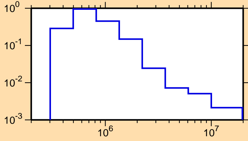
\sigma vs. E for ^{244}\text{Cf}(n,n_2)
