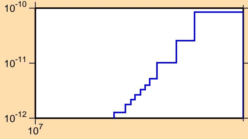
\sigma vs. E for ^{245}\text{Cf}(n,p\alpha)
