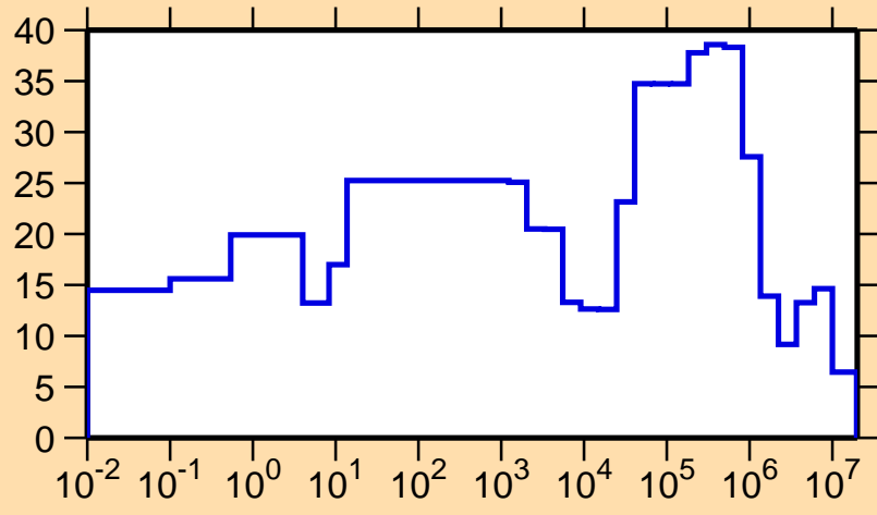
\Delta\sigma/\sigma vs. E for ^{245}\text{Cf}(n,el.)
