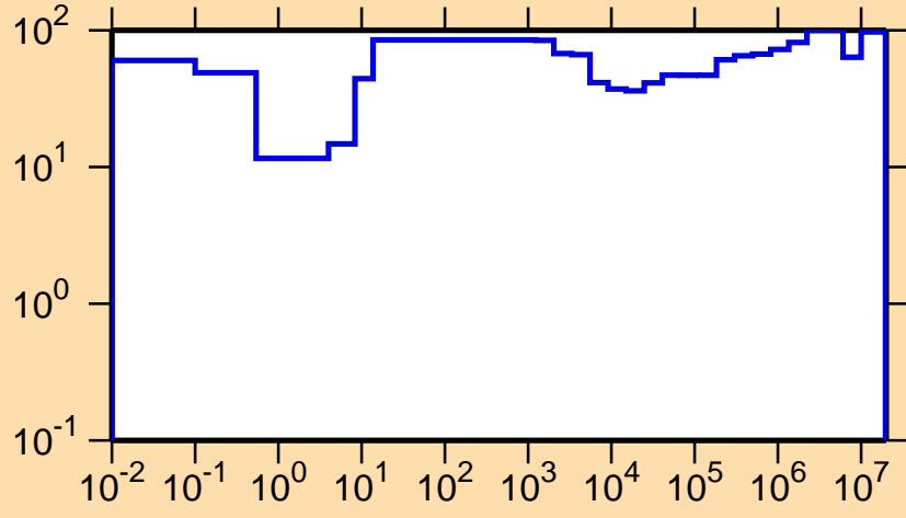
\Delta\sigma/\sigma vs. E for ^{245}\text{Cf}(n,\gamma)
