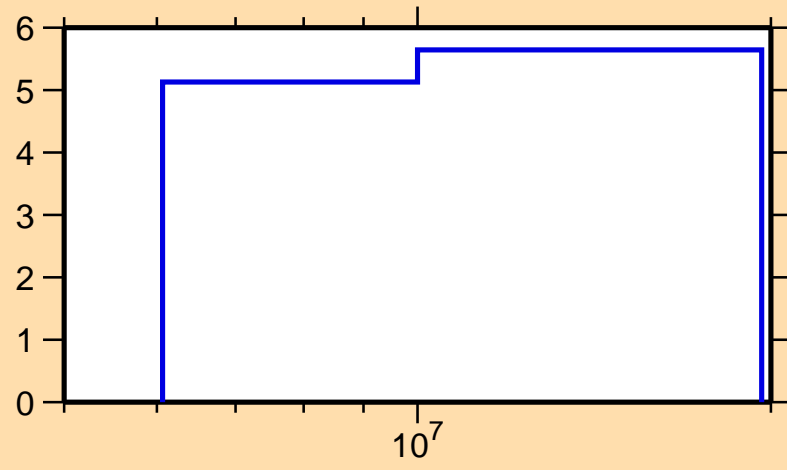
\Delta\sigma/\sigma vs. E for ^{245}\text{Cf}(n,\text{tot.})
