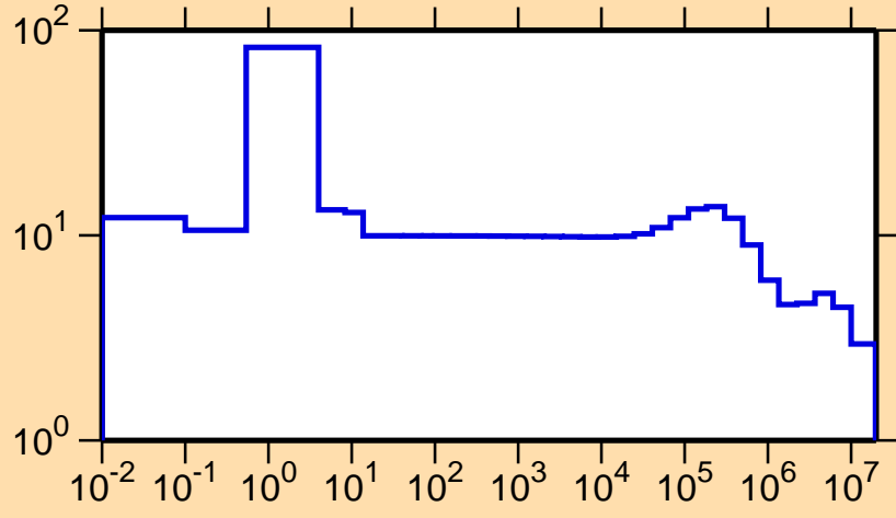
\sigma vs. E for ^{245}\text{Cf}(n,\text{el.})
