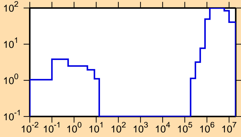
\Delta\sigma/\sigma vs. E for ^{245}\text{Cf}(n,p)
