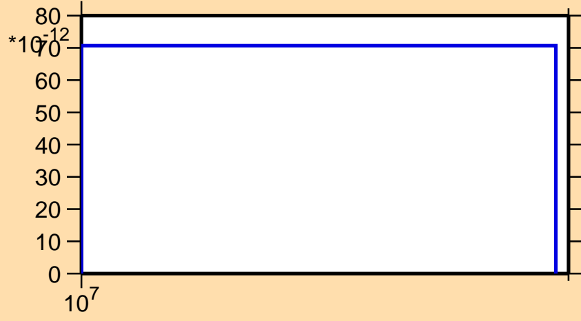
\sigma vs. E for ^{245}\text{Cf}(n,nt)
