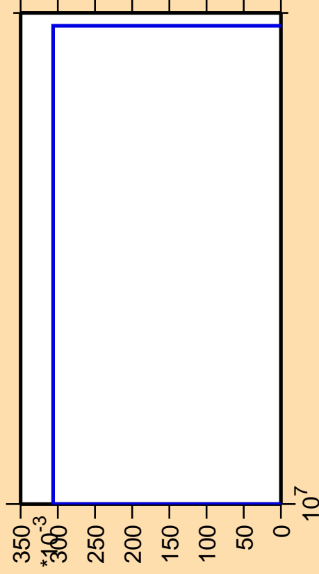
\Delta\sigma/\sigma vs. E for ^{245}\text{Cf}(\text{mt117})
