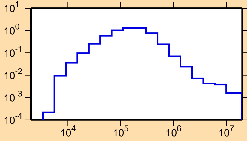
\sigma vs. E for ^{245}\text{Cf}(n,n_1)
