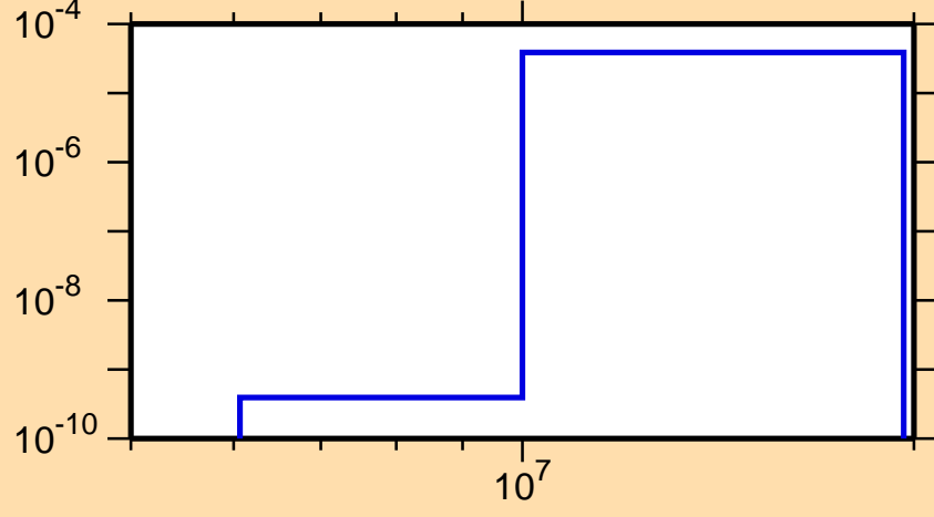
\sigma vs. E for ^{245}\text{Cf}(n,np)
