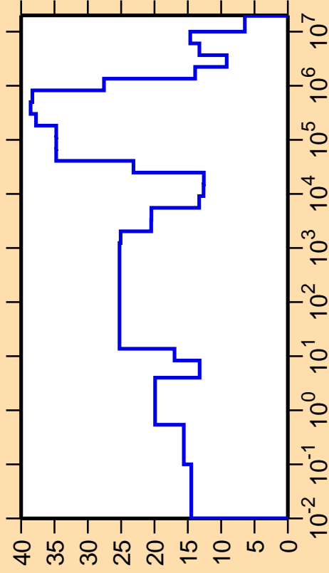
\Delta\sigma/\sigma vs. E for ^{245}\text{Cf}(n,\text{el.})
