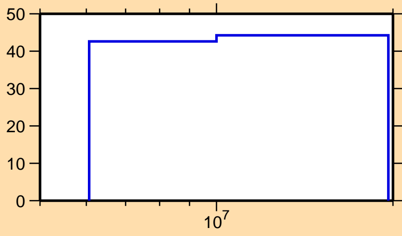
\Delta\sigma/\sigma vs. E for ^{245}\text{Cf}(n,2n)
