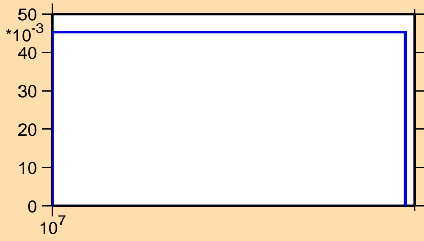
\sigma vs. E for ^{245}\text{Cf}(n,3n)
