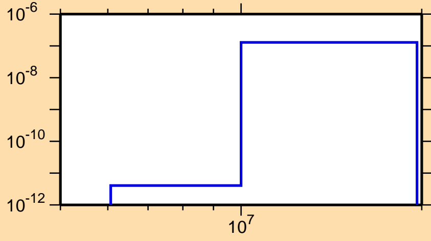
\sigma vs. E for ^{245}\text{Cf}(n,2n\alpha)
