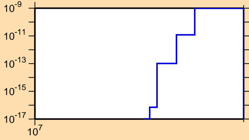
\sigma vs. E for ^{246}\text{Cf}(n,2np)
