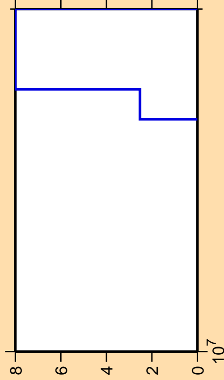
\Delta\sigma/\sigma vs. E for ^{246}\text{Cf}(n,p\alpha)
