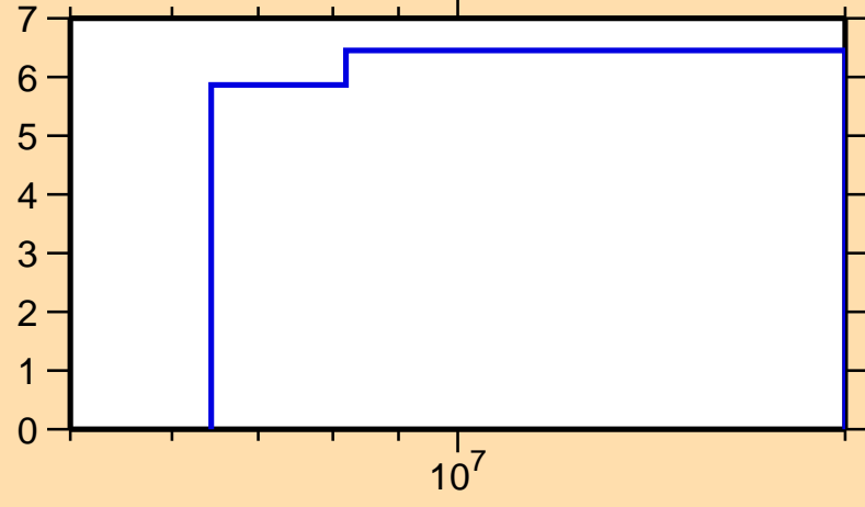
\Delta\sigma/\sigma vs. E for ^{246}\text{Cf}(n,\text{nonel.})
