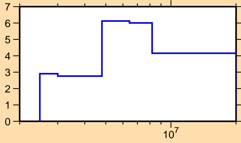
\Delta\sigma/\sigma vs. E for ^{246}\text{Cf}(n,\text{tot.})
