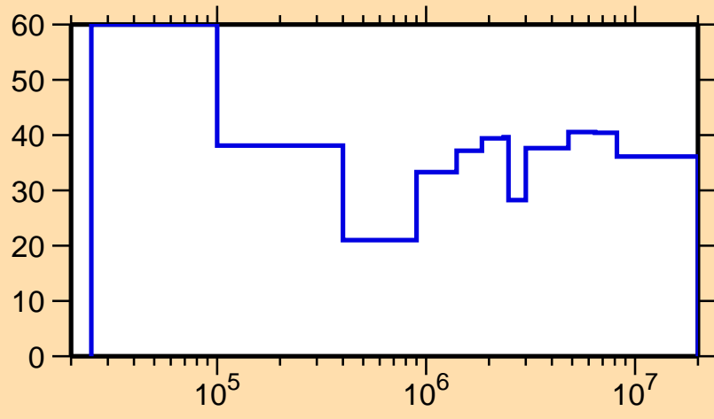
\Delta\sigma/\sigma vs. E for ^{246}\text{Cf}(n,n_1)
