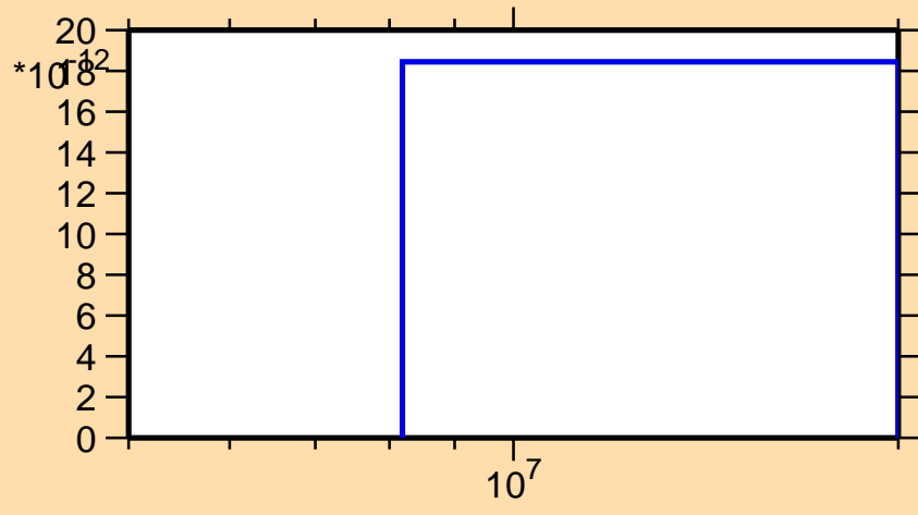
\sigma vs. E for ^{246}\text{Cf}(n,nd)
