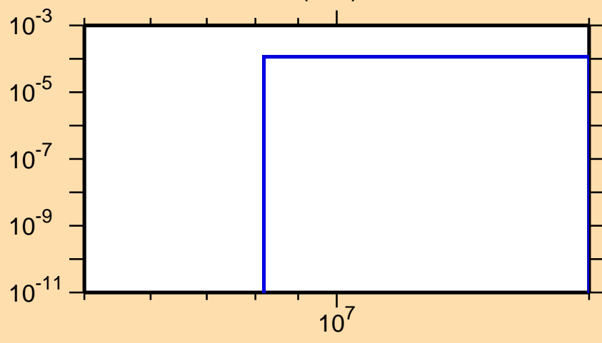
\sigma vs. E for ^{246}\text{Cf}(n,d)
