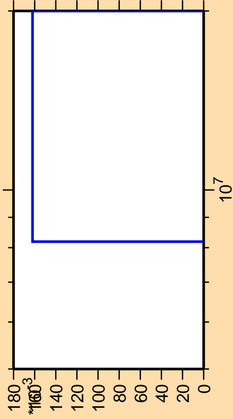
\Delta\sigma/\sigma vs. E for ^{246}\text{Cf}(n,p\alpha)
