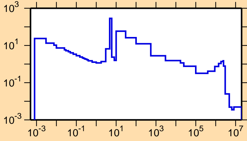
\sigma vs. E for ^{246}\text{Cf}(n,\gamma)
