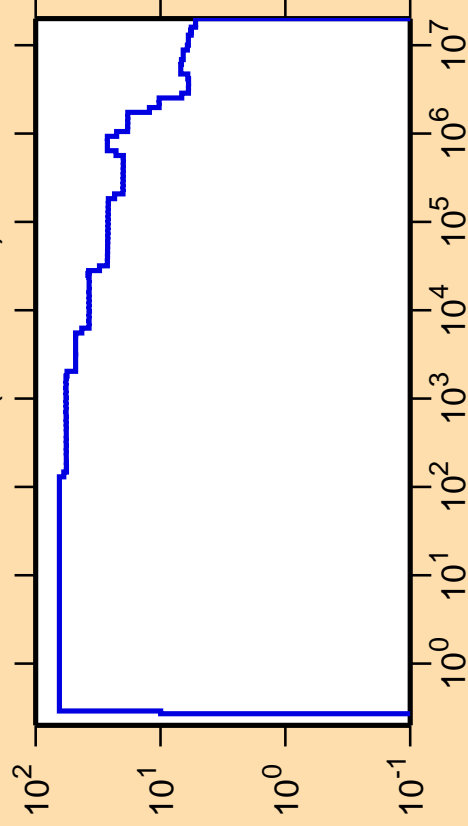
\Delta\sigma/\sigma vs. E for ^{247}\text{Cf}(n,\text{nonel.})
