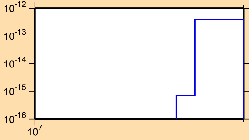
\sigma vs. E for ^{247}\text{Cf} (mt 34)
