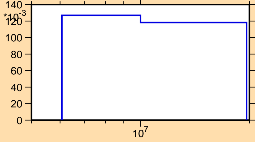
\sigma vs. E for ^{247}\text{Cf}(n,2n)
