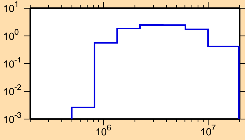
\sigma vs. E for ^{247}\text{Cf}(n,n\text{cont.})
