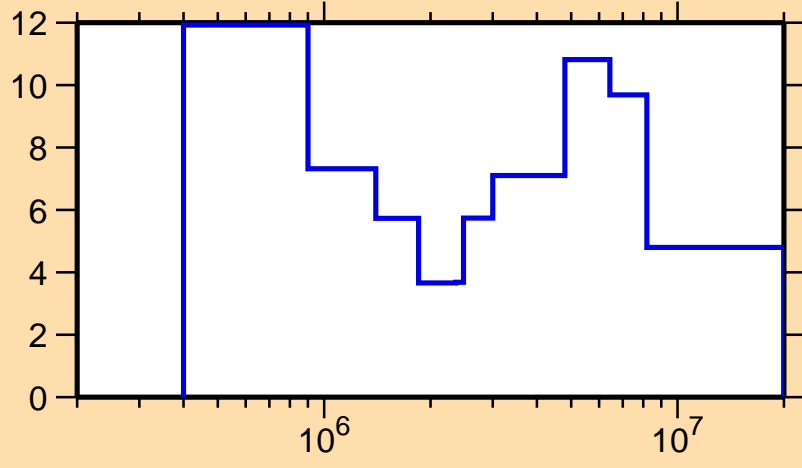
\Delta\sigma/\sigma vs. E for ^{247}\text{Cf}(n,tot.)
