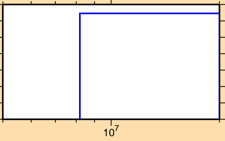
\sigma vs. E for ^{247}\text{Cf}(n,3n)
