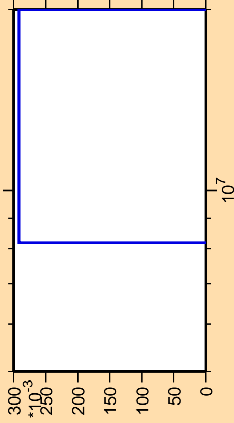
\Delta\sigma/\sigma vs. E for ^{247}\text{Cf}(n,p\alpha)
