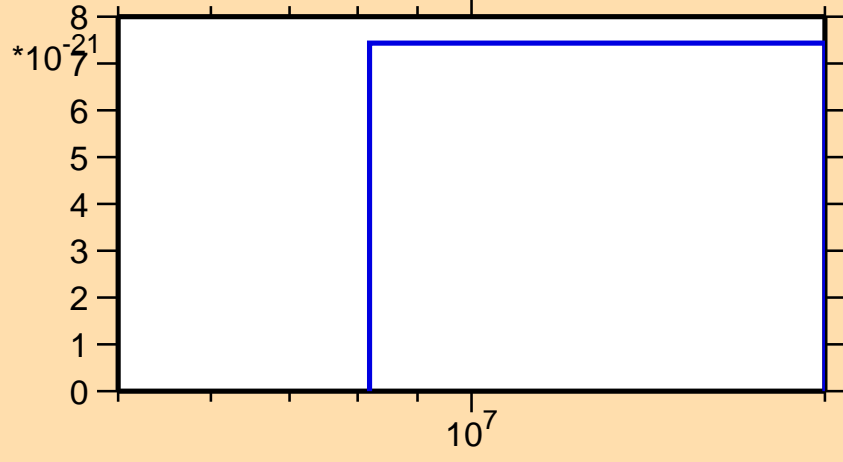
\sigma vs. E for ^{247}\text{Cf}(\text{mt } 42)
