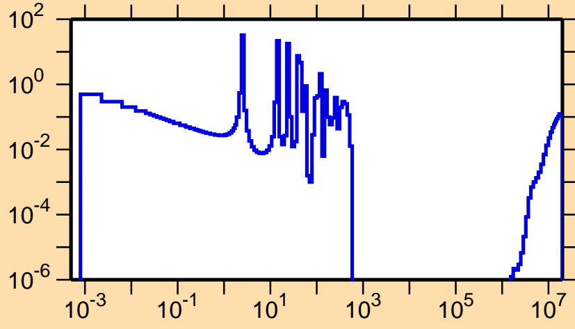
\sigma vs. E for ^{248}\text{Cf}(n,f)
