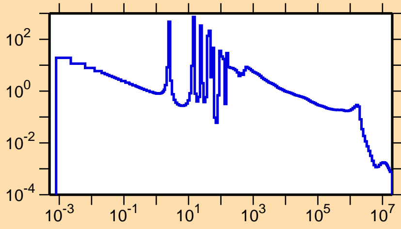
\sigma vs. E for ^{248}\text{Cf}(n,\gamma)
