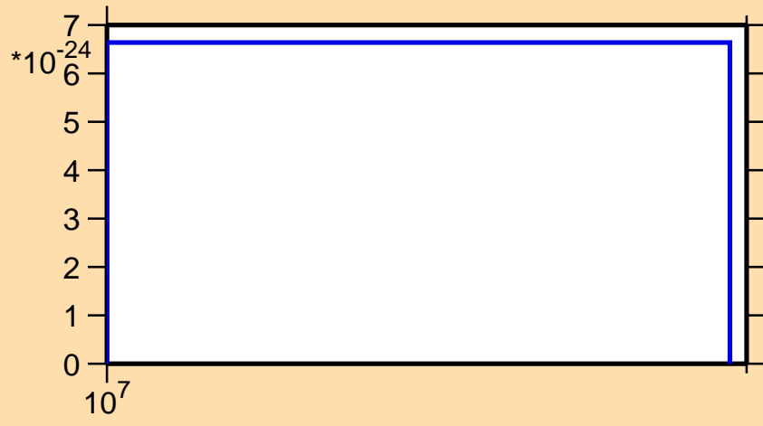
\sigma vs. E for ^{248}\text{Cf} (mt 42)
