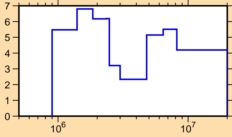
\Delta\sigma/\sigma vs. E for ^{249}\text{Cf}(n,inel.)
