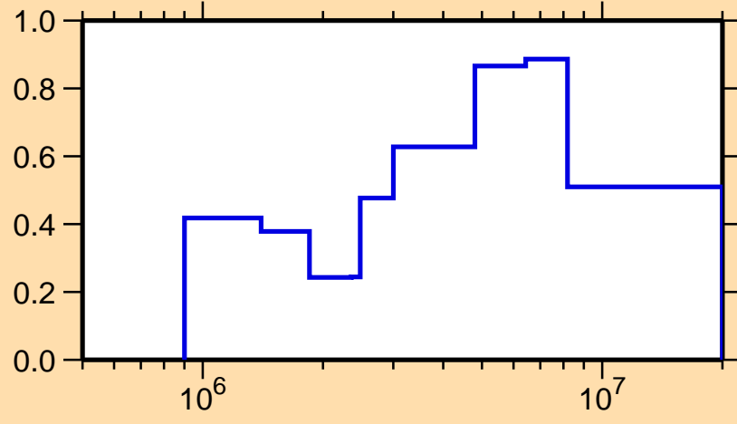
\Delta\sigma/\sigma vs. E for ^{249}\text{Cf}(n,tot.)
