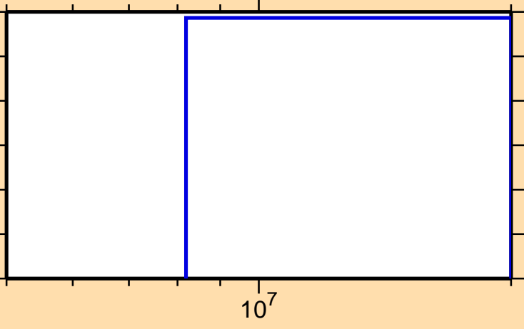
\sigma vs. E for ^{251}\text{Cf}(n,nt)
