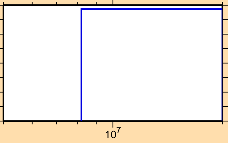
\sigma vs. E for ^{251}\text{Cf}(n,2n\alpha)
