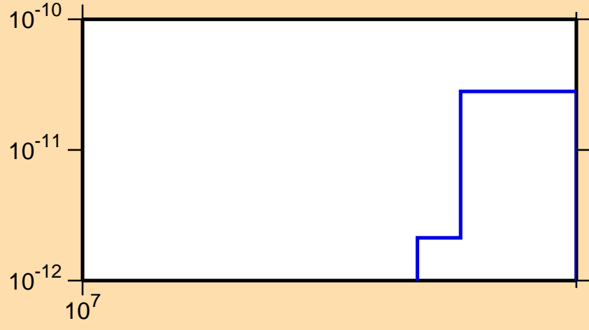
\sigma vs. E for ^{252}\text{Cf}(n,3n\alpha)
