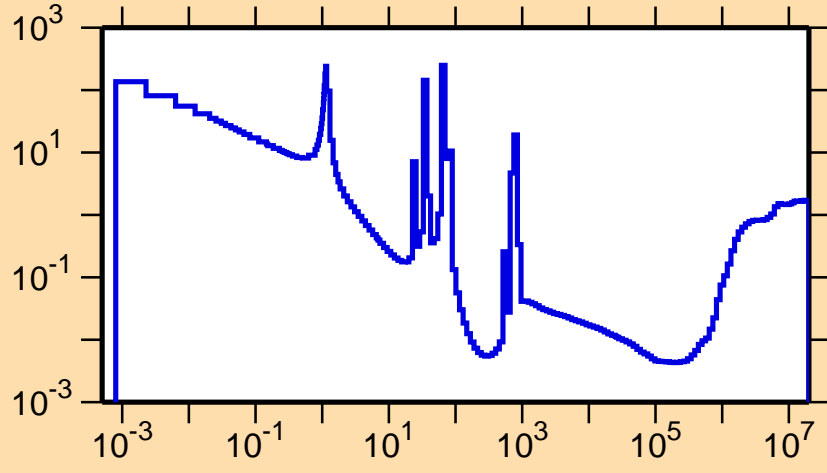
\sigma vs. E for ^{252}\text{Cf}(n,f)
