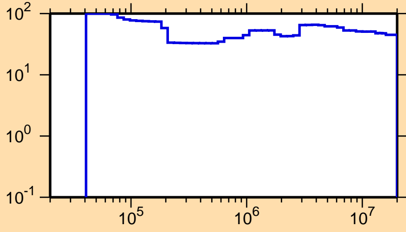
\Delta\sigma/\sigma vs. E for ^{252}\text{Cf}(n,n_1)
