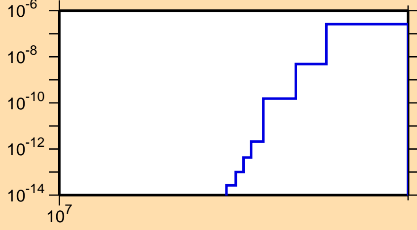
\sigma vs. E for ^{252}\text{Cf}(n,nd)
