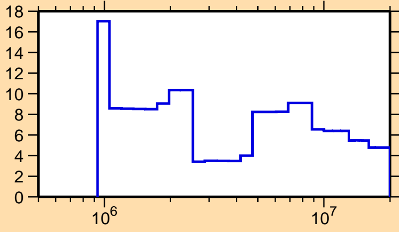
\Delta\sigma/\sigma vs. E for ^{252}\text{Cf}(n,\text{tot.})
