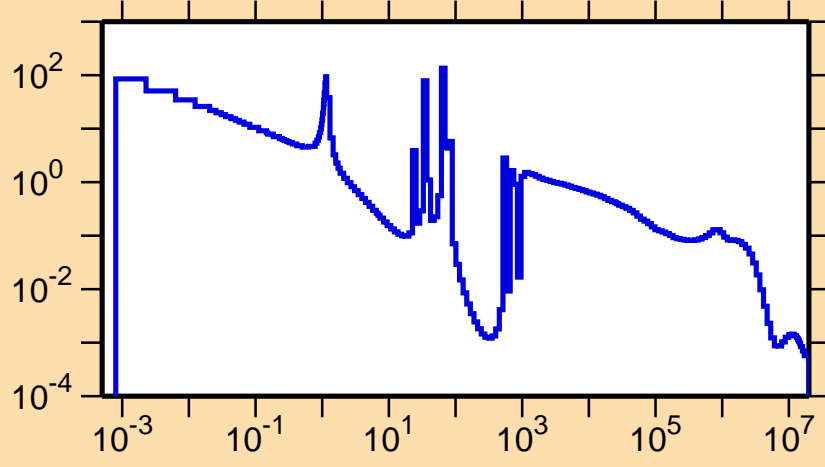
\sigma vs. E for ^{252}\text{Cf}(n,\gamma)
