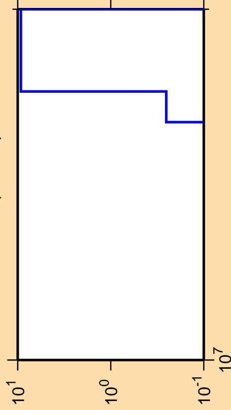
\Delta\sigma/\sigma vs. E for ^{252}\text{Cf}(n,\text{He3})
