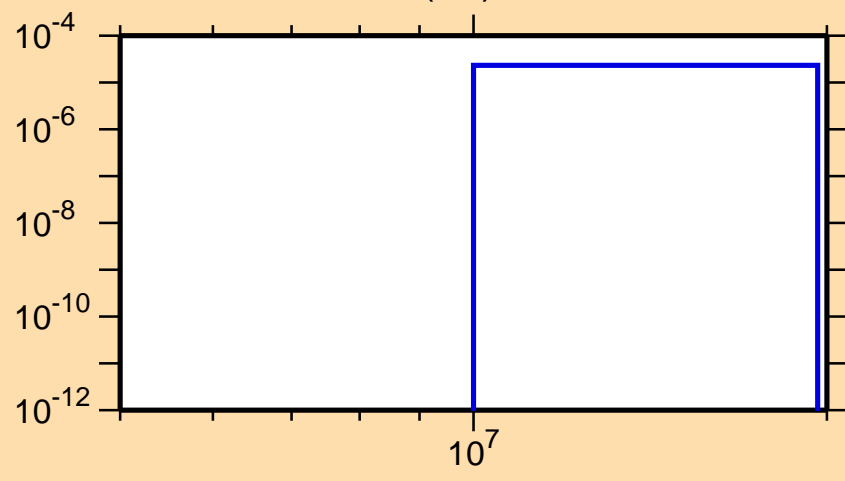
\sigma vs. E for ^{252}\text{Cf}(n,t)
