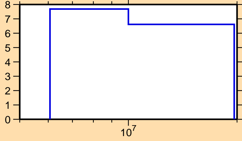
\Delta\sigma/\sigma vs. E for ^{252}\text{Cf}(n,\text{nonel.})
