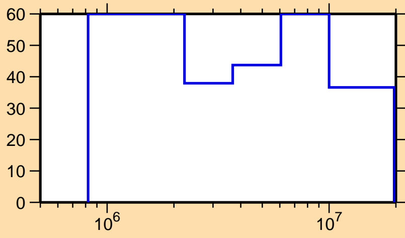
\Delta\sigma/\sigma vs. E for ^{252}\text{Cf}(n,n\text{cont.})
