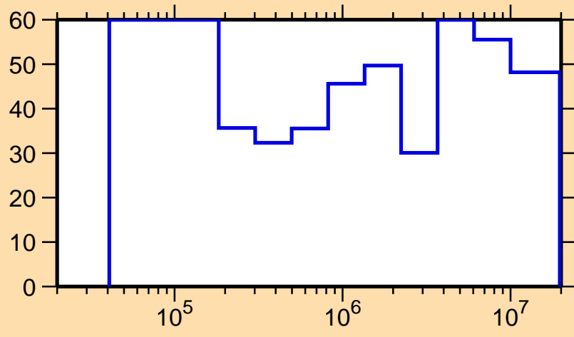
\Delta\sigma/\sigma vs. E for ^{252}\text{Cf}(n,n_1)
