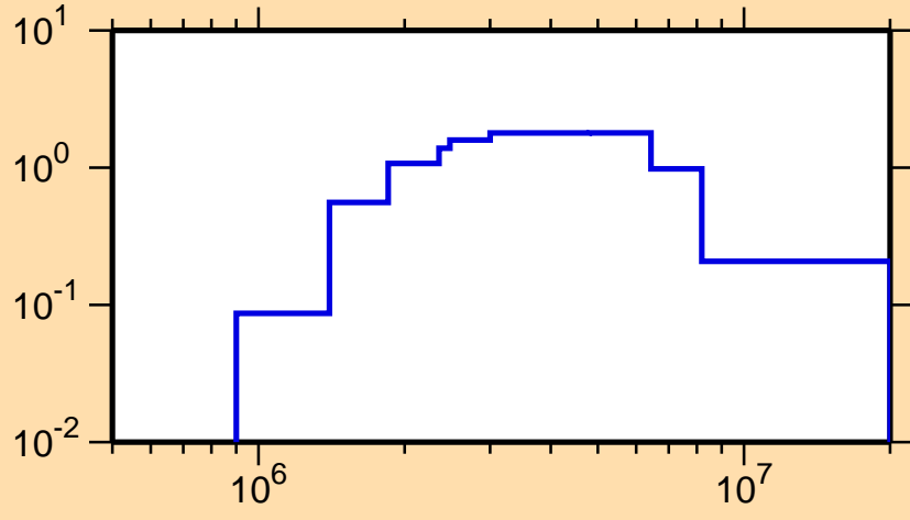
\sigma vs. E for ^{252}\text{Cf}(n,n\text{cont.})
