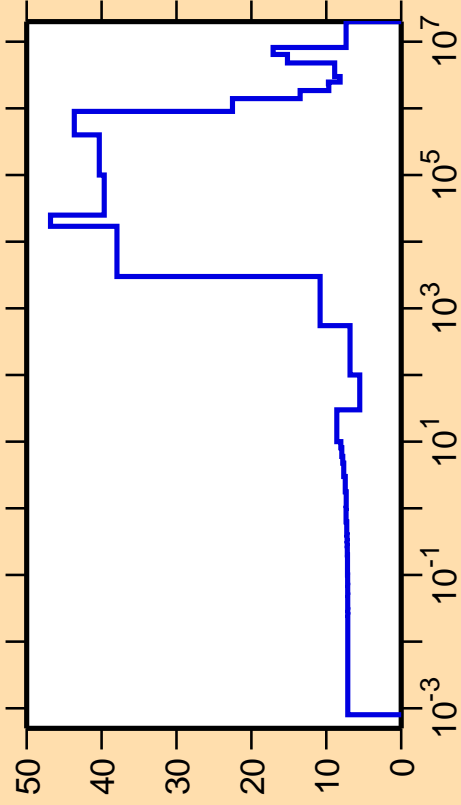
\Delta\sigma/\sigma vs. E for ^{252}\text{Cf}(n,\text{el.})
