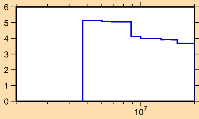
\Delta\sigma/\sigma vs. E for ^{253}\text{Cf}(n,\text{nonel.})
