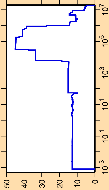
\Delta\sigma/\sigma vs. E for ^{253}\text{Cf}(n,\text{el.})
