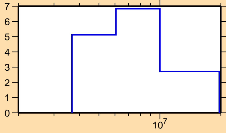
\Delta\sigma/\sigma vs. E for ^{253}\text{Cf}(n,\text{tot.})
