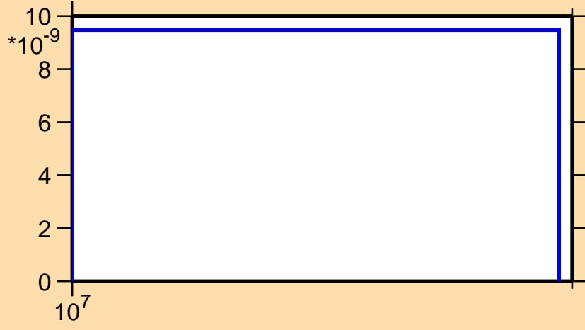
\sigma vs. E for ^{253}\text{Cf}(n,nd)
