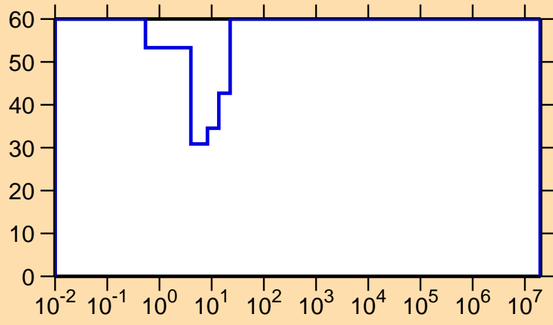
\Delta\sigma/\sigma vs. E for ^{253}\text{Cf}(n,\gamma)
