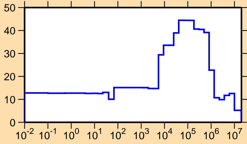
\Delta\sigma/\sigma vs. E for ^{253}\text{Cf}(n,el.)
