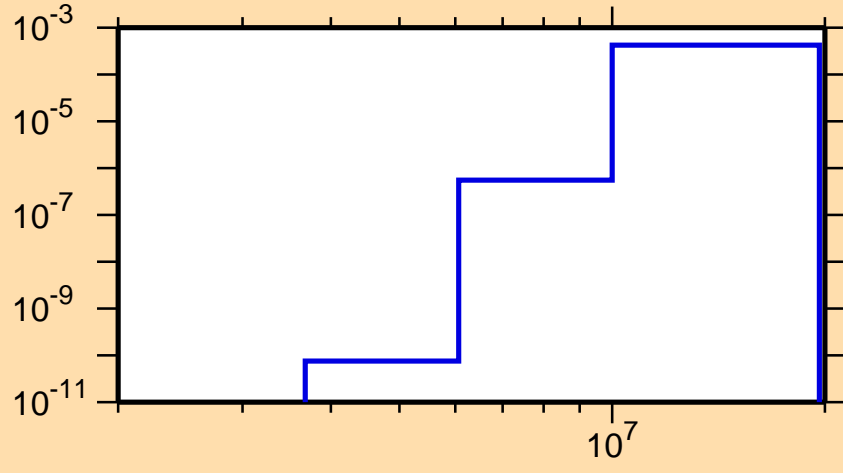
\sigma vs. E for ^{253}\text{Cf}(n,p)
