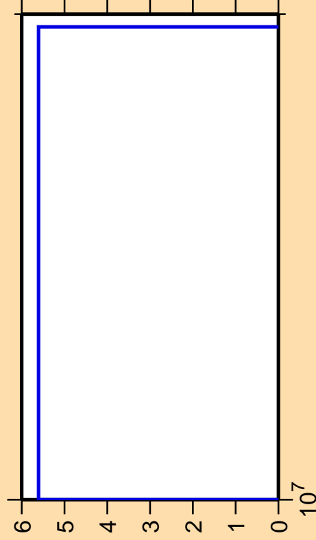
\Delta\sigma/\sigma vs. E for ^{254}\text{Cf}(n,3n\alpha)
