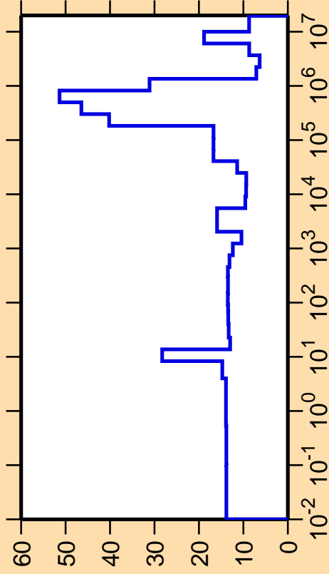
\Delta\sigma/\sigma vs. E for ^{254}\text{Cf}(n,\text{el.})
