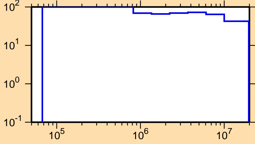
\Delta\sigma/\sigma vs. E for ^{254}\text{Cf}(n, ncont.)
