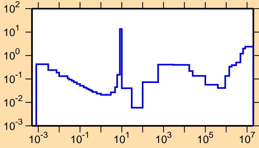
\sigma vs. E for ^{254}\text{Cf}(n,f)
