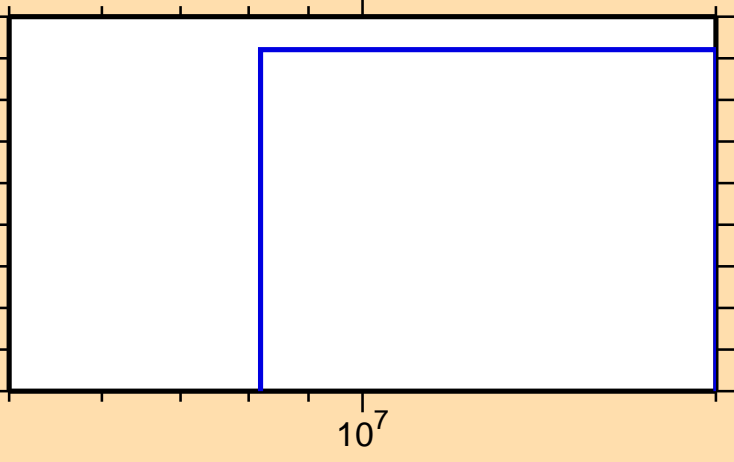
\sigma vs. E for ^{254}\text{Cf}(n,t)
