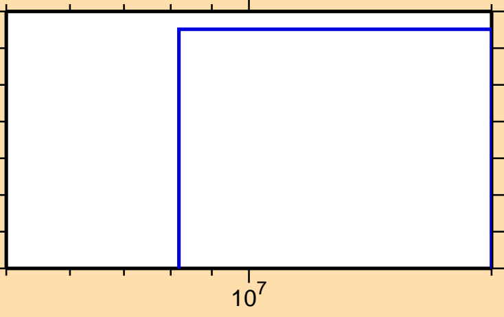
\sigma vs. E for ^{254}\text{Cf}(n,d)
