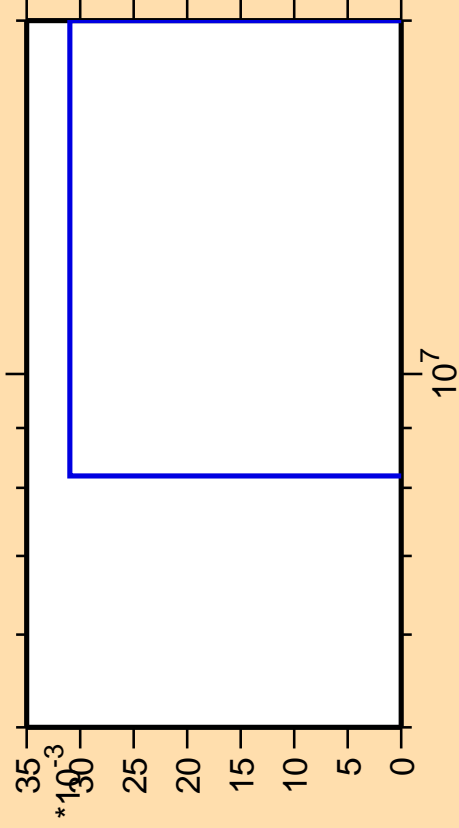
\Delta\sigma/\sigma vs. E for ^{254}\text{Cf}(n,\text{He3})
