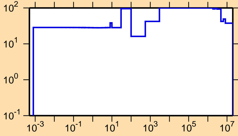
\Delta\sigma/\sigma vs. E for ^{254}\text{Cf}(n,f)
