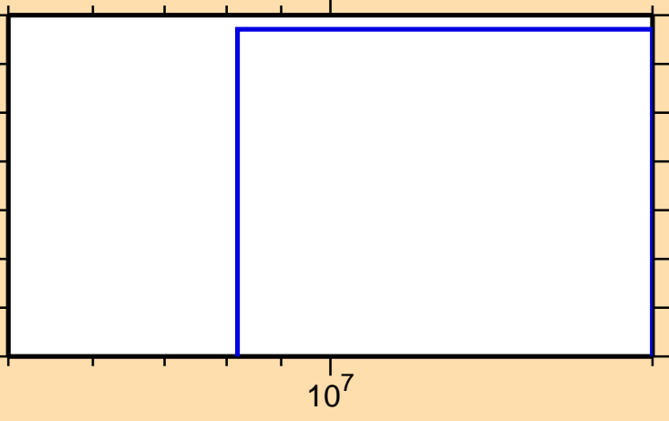
\sigma vs. E for ^{254}\text{Cf}(n,nt)
