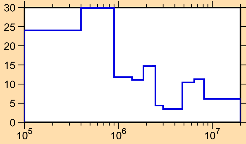
\Delta\sigma/\sigma vs. E for ^{254}\text{Cf}(n, tot.)
