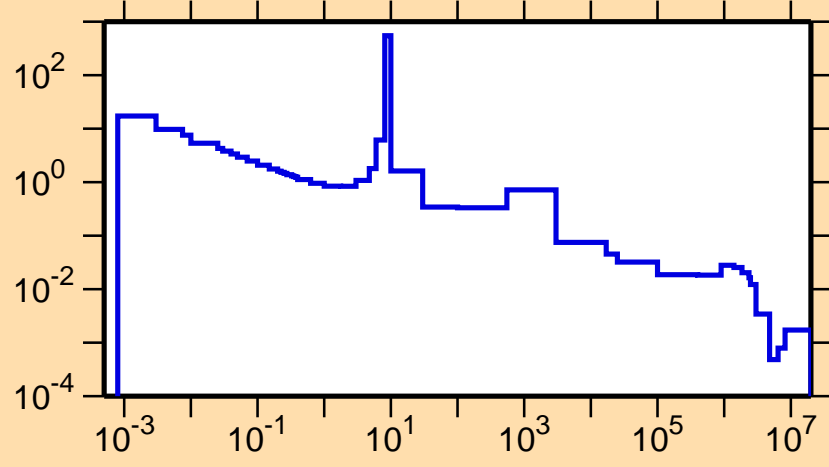
\sigma vs. E for ^{254}\text{Cf}(n,\gamma)
