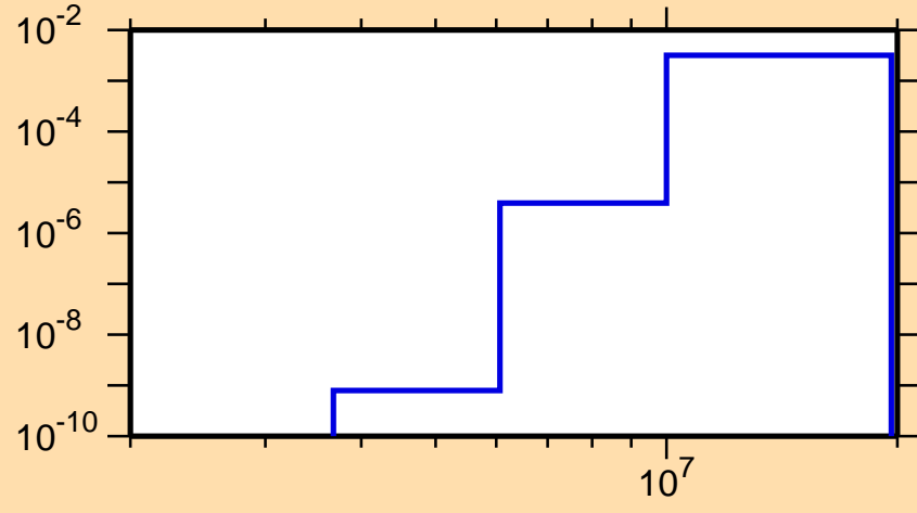
\sigma vs. E for ^{255}\text{Cf}(n,p)
