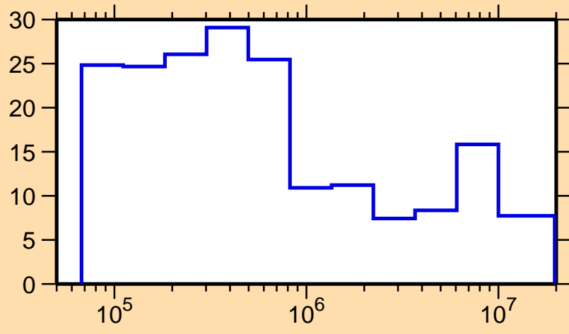
\Delta\sigma/\sigma vs. E for ^{255}\text{Cf}(n,\text{tot.})
