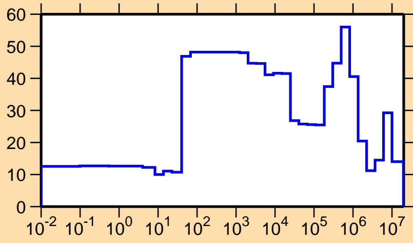
\Delta\sigma/\sigma vs. E for ^{255}\text{Cf}(n,el.)
