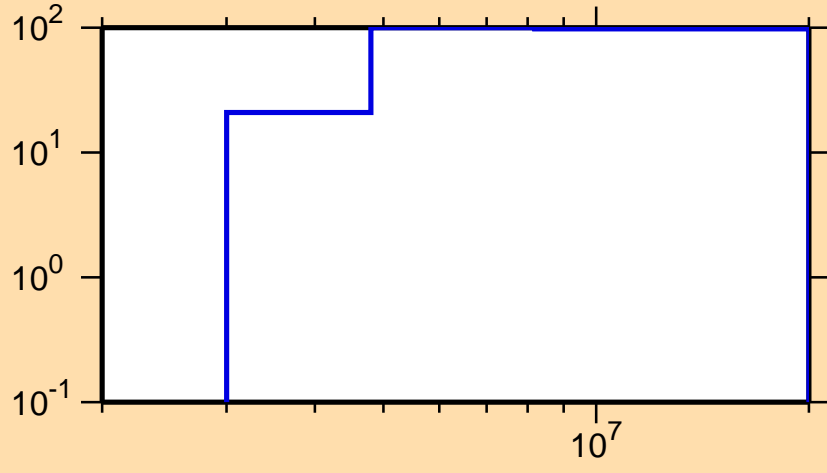
\Delta\sigma/\sigma vs. E for ^{255}\text{Cf}(n,p)
