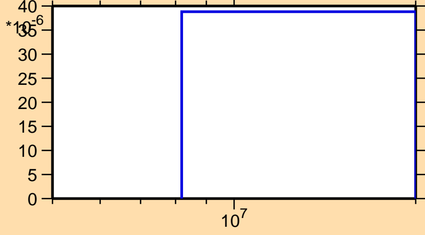
\sigma vs. E for ^{255}\text{Cf}(n,d)
