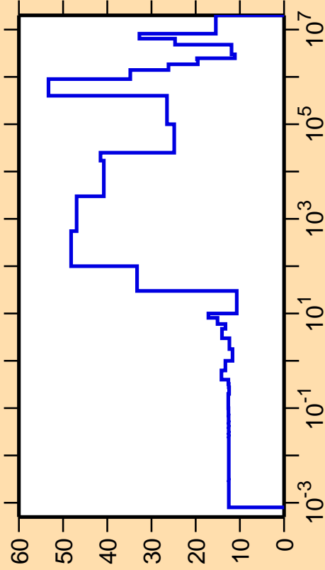
\Delta\sigma/\sigma vs. E for ^{255}\text{Cf}(n,\text{el.})
