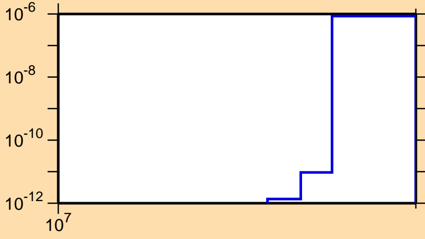
\sigma vs. E for ^{34}\text{Cl} (mt 34)
