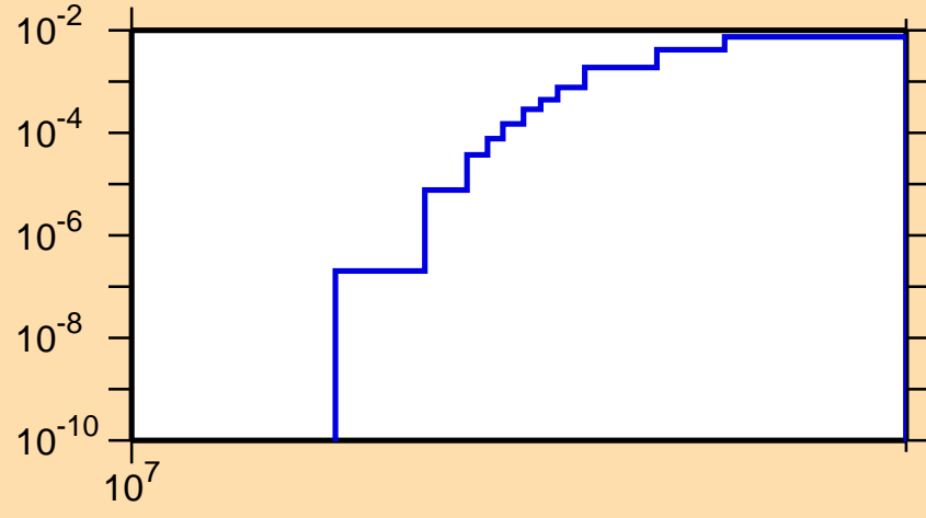
\sigma vs. E for ^{34}\text{Cl}(n,nd)
