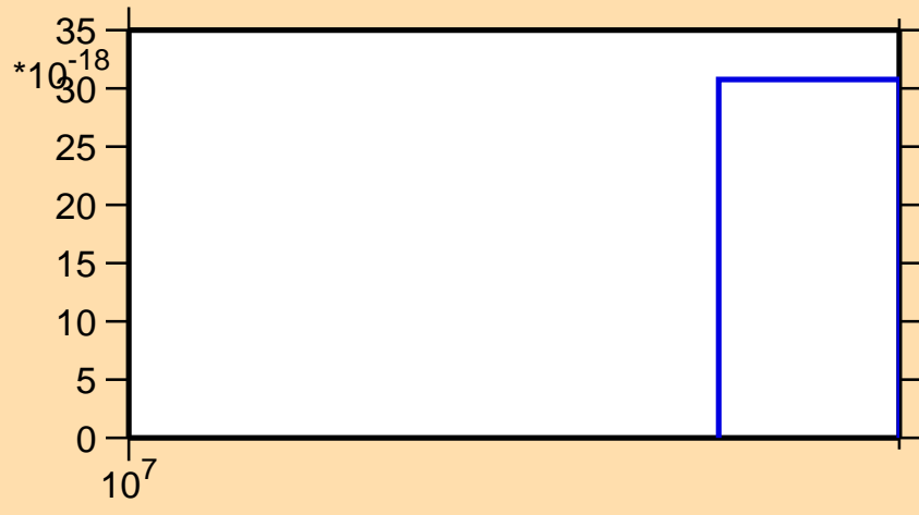
\sigma vs. E for ^{34}\text{Cl}(n,2n\alpha)
