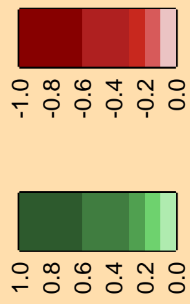
Correlation Matrix
