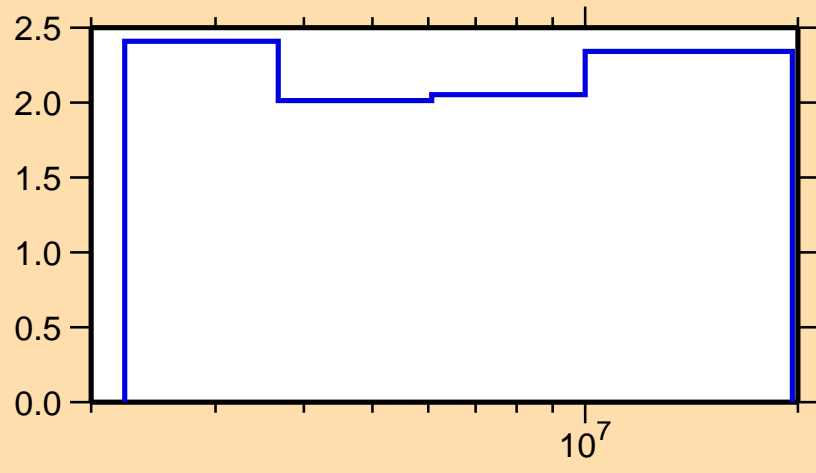
\Delta\sigma/\sigma vs. E for ^{34}\text{Cl}(n,n\text{onel.})
