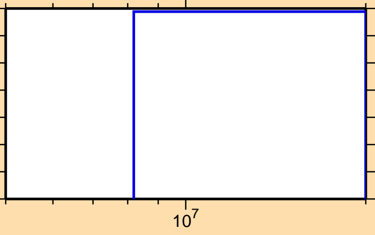
\sigma vs. E for ^{34}\text{Cl}(\text{mt } 45)
