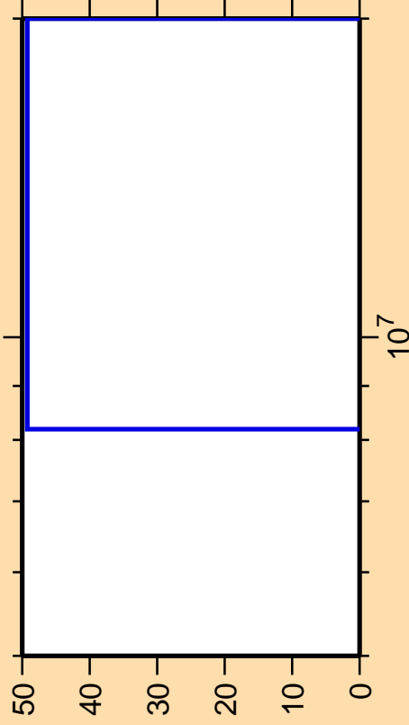
\Delta\sigma/\sigma vs. E for ^{34}\text{Cl}(\text{mt117})
