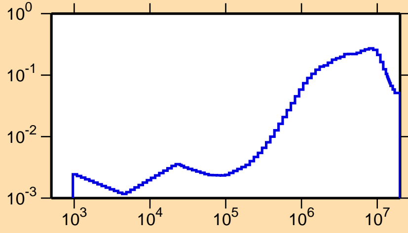
\sigma vs. E for ^{35}\text{Cl}(n,p)
