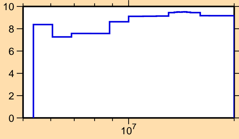
\Delta\sigma/\sigma vs. E for ^{35}\text{Cl}(n,ncont.)
