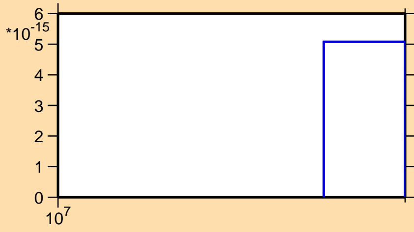
\sigma vs. E for ^{35}\text{Cl}(n,\text{pt})
