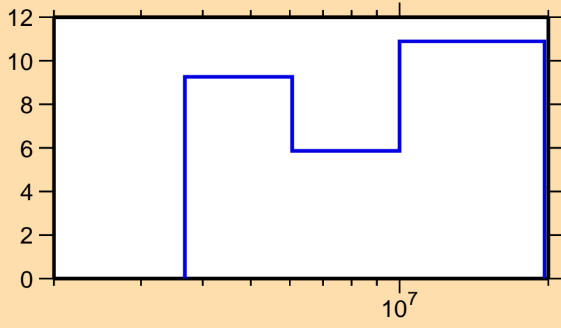
\Delta\sigma/\sigma vs. E for ^{36}\text{Cl}(n,ncont.)
