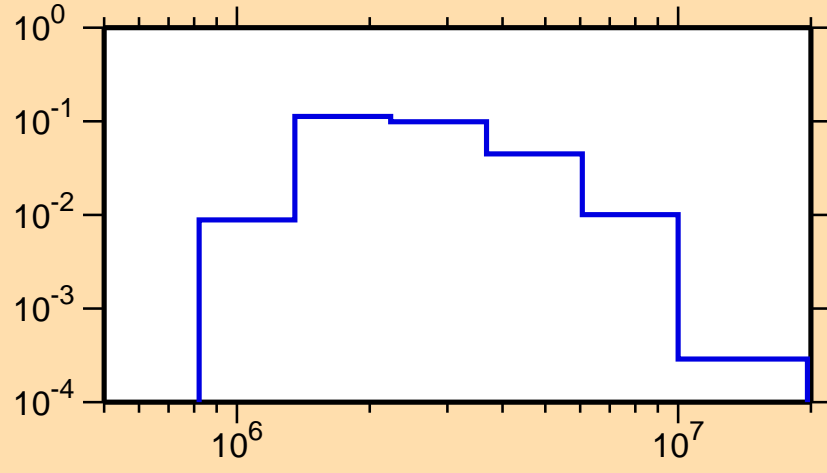
\sigma vs. E for ^{36}\text{Cl}(n,n_2)
