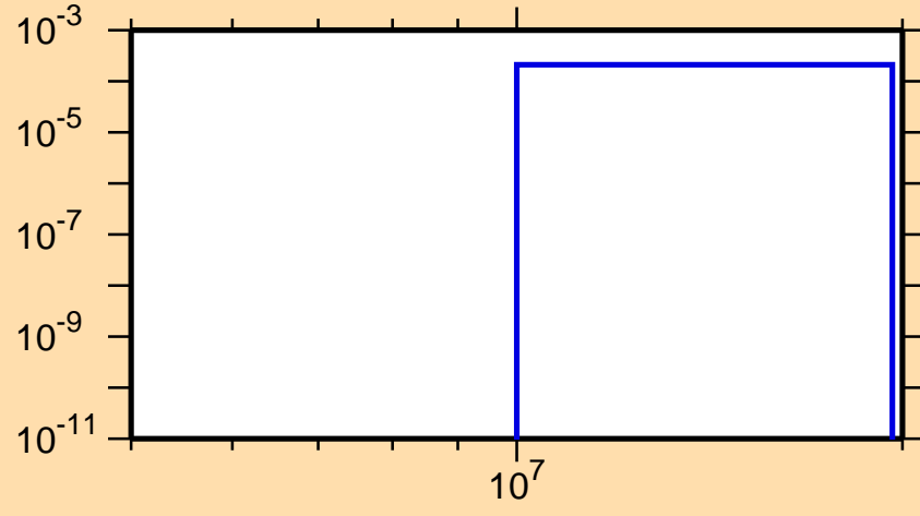
\sigma vs. E for ^{36}\text{Cl}(n,p\alpha)
