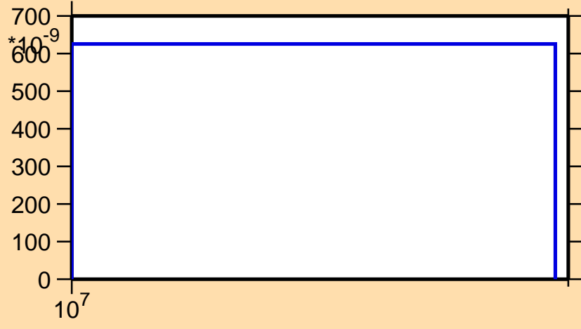
\sigma vs. E for ^{36}\text{Cl}(n,\text{He}3)
