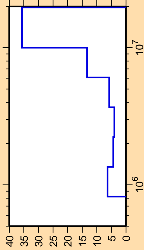
\Delta\sigma/\sigma vs. E for ^{36}\text{Cl}(n,n_2)
