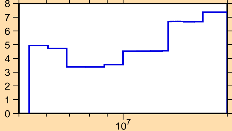
\Delta\sigma/\sigma vs. E for ^{37}\text{Cl}(n,n\text{cont.})
