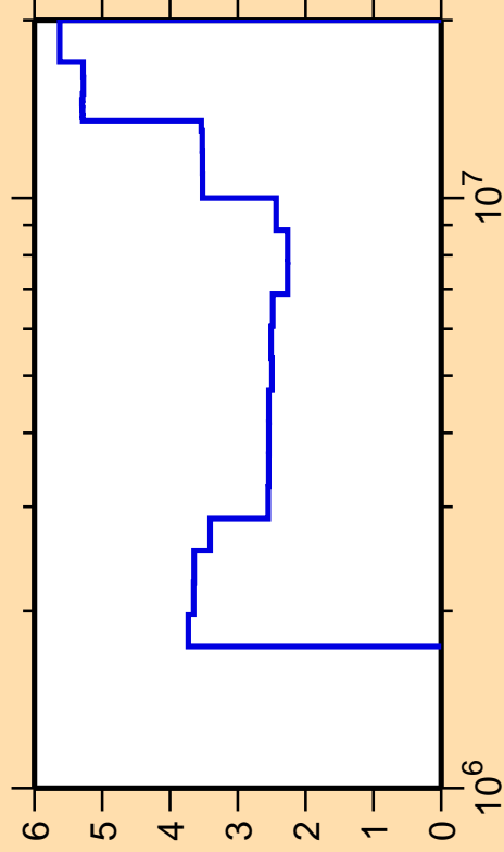
\Delta\sigma/\sigma vs. E for ^{37}\text{Cl}(n,\text{inel.})
