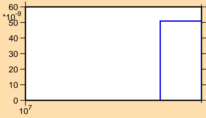
\sigma vs. E for ^{37}\text{Cl}(n,2np)
