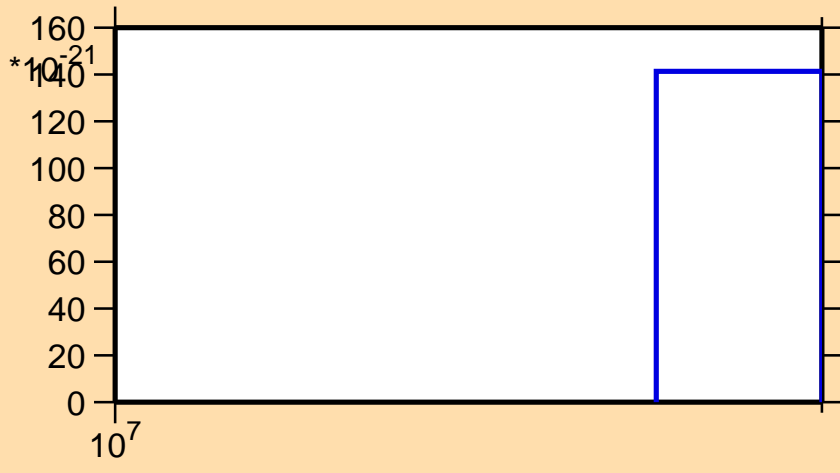
\sigma vs. E for ^{37}\text{Cl}(n,\text{pd})
