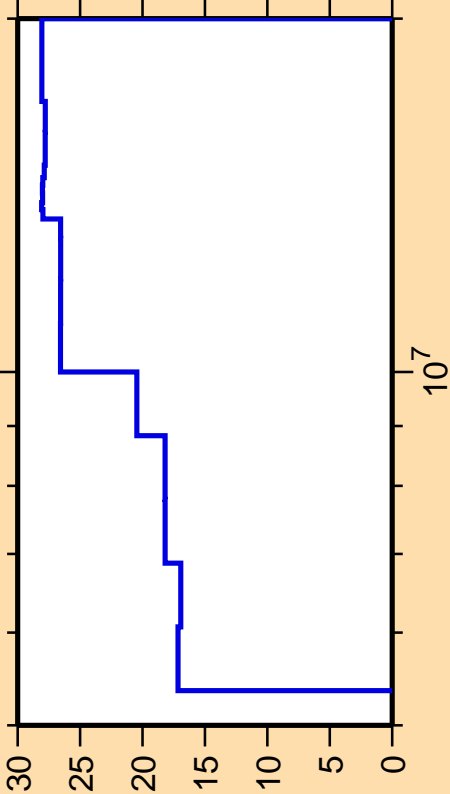
\Delta\sigma/\sigma vs. E for ^{37}\text{Cl}(n,\gamma)
