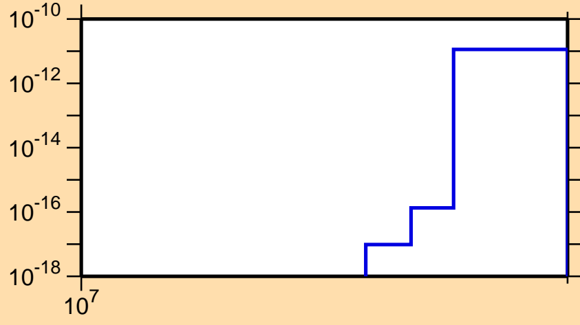
\sigma vs. E for ^{37}\text{Cl}(\text{mt117})
