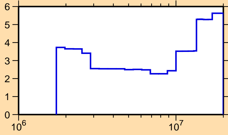
\Delta\sigma/\sigma vs. E for ^{37}\text{Cl}(n,\text{inel.})
