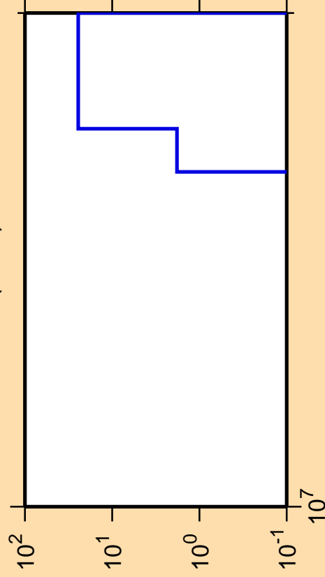
\Delta\sigma/\sigma vs. E for ^{37}\text{Cl}(n,nd)
