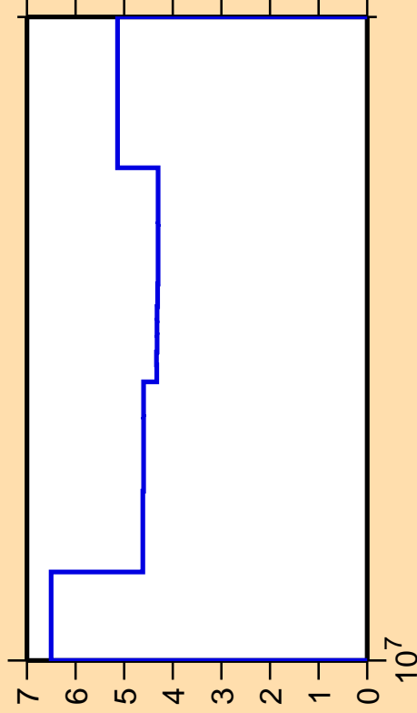
\Delta\sigma/\sigma vs. E for ^{37}\text{Cl}(n,2n)
