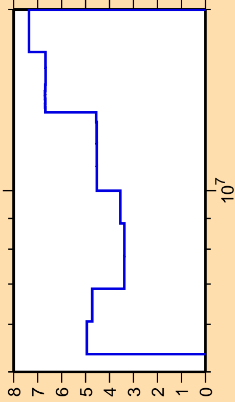
\Delta\sigma/\sigma vs. E for ^{37}\text{Cl}(n,n\text{cont.})
