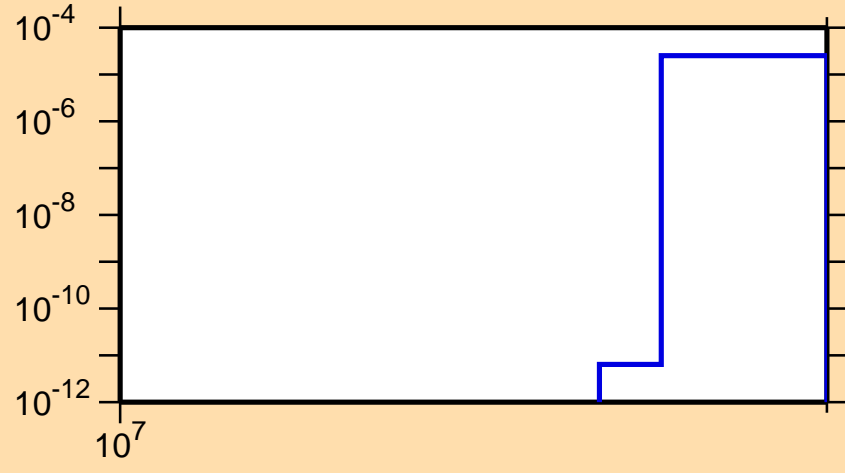
\sigma vs. E for ^{37}\text{Cl}(n,nd)
