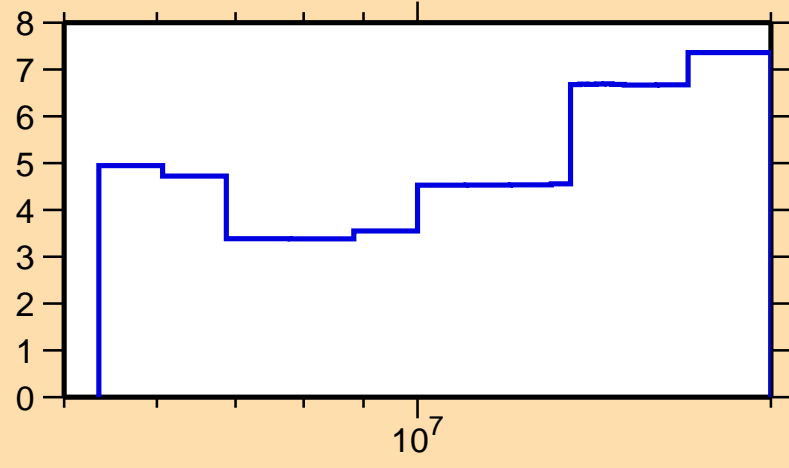
\Delta\sigma/\sigma vs. E for ^{37}\text{Cl}(n,n\text{cont.})
