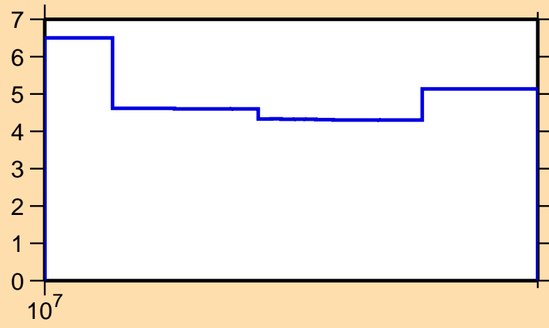
\Delta\sigma/\sigma vs. E for ^{37}\text{Cl}(n,2n)
