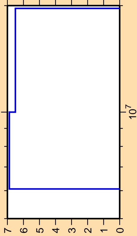
\Delta\sigma/\sigma vs. E for ^{37}\text{Cl}(n,np)
