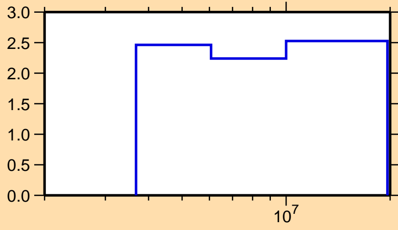
\Delta\sigma/\sigma vs. E for ^{37}\text{Cl}(n,n\text{onel.})
