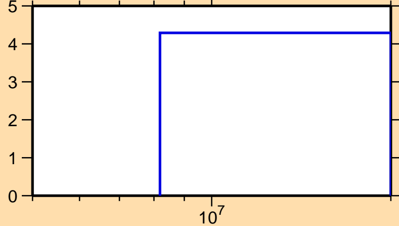
\Delta\sigma/\sigma vs. E for ^{37}\text{Cl}(n,2n)
