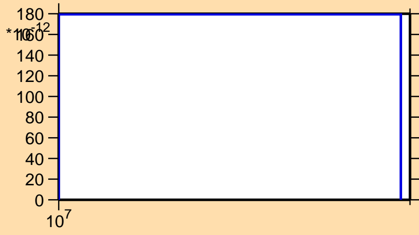
\sigma vs. E for ^{39}\text{Cl}(n,2n\alpha)
