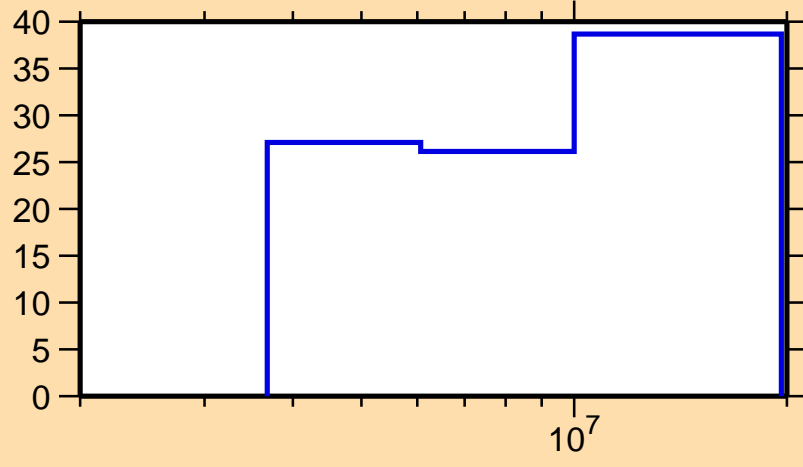
\Delta\sigma/\sigma vs. E for ^{39}\text{Cl}(n,\gamma)
