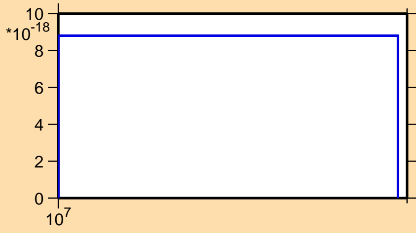
\sigma vs. E for ^{39}\text{Cl}(n,\text{He}3)
