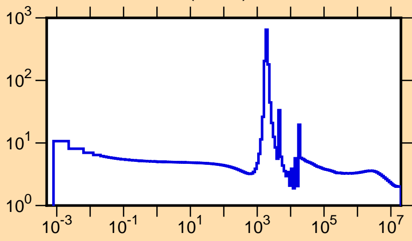
\sigma vs. E for ^{40}\text{Cl}(n,\text{tot.})
