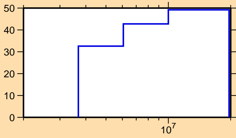
\Delta\sigma/\sigma vs. E for ^{40}\text{Cl}(n,\gamma)
