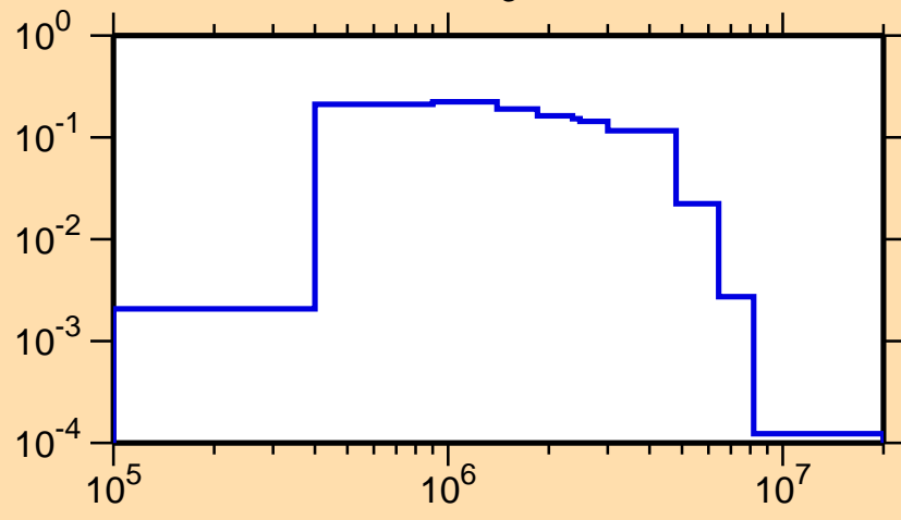
\sigma vs. E for ^{40}\text{Cl}(n,n_3)
