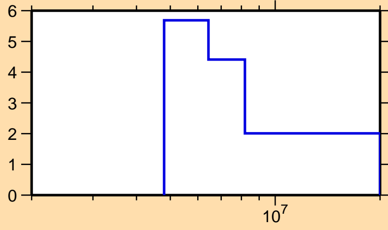
\Delta\sigma/\sigma vs. E for ^{40}\text{Cl}(n,2n)
