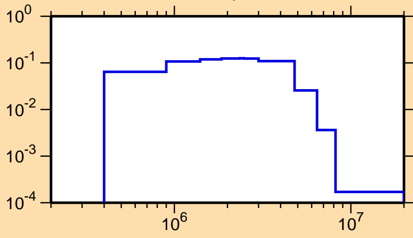
\sigma vs. E for ^{40}\text{Cl}(n,n_4)
