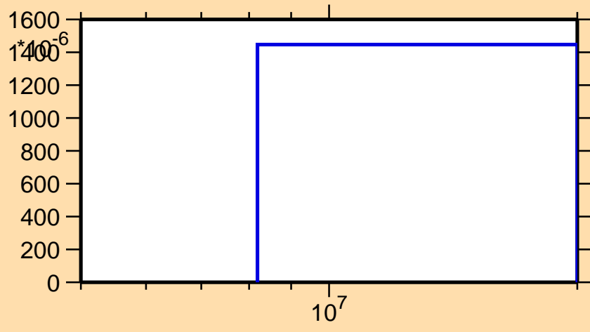
\sigma vs. E for ^{40}\text{Cl}(n,d)
