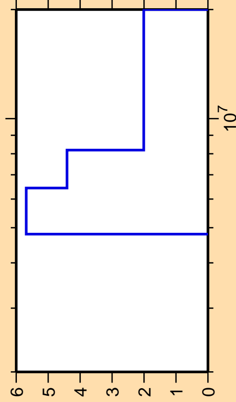
\Delta\sigma/\sigma vs. E for ^{40}\text{Cl}(n,2n)
