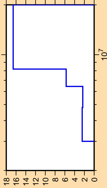
\Delta\sigma/\sigma vs. E for ^{40}\text{Cl}(n,\text{ncont.})
