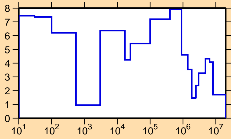
\Delta\sigma/\sigma vs. E for ^{40}\text{Cl}(n,\text{el.})
