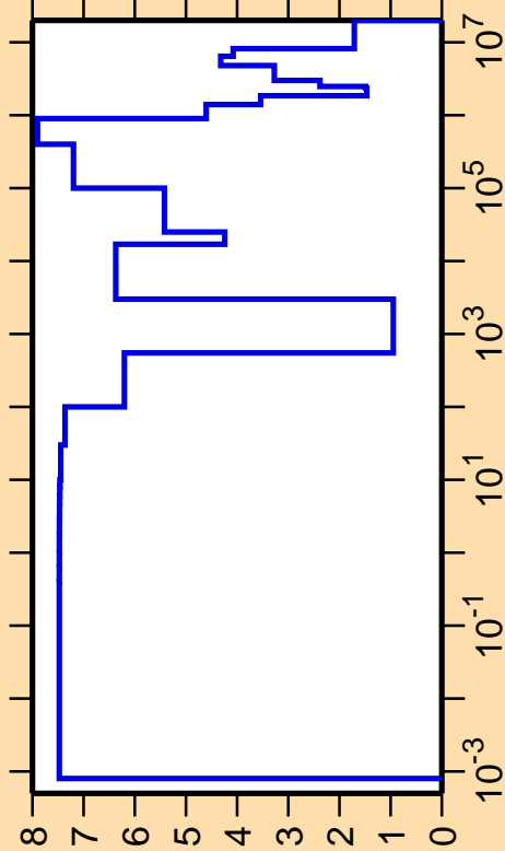
\Delta\sigma/\sigma vs. E for ^{40}\text{Cl}(n,\text{el.})
