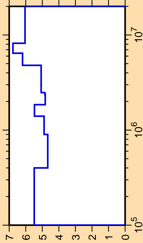
\Delta\sigma/\sigma vs. E for ^{40}\text{Cl}(n,n_2)
