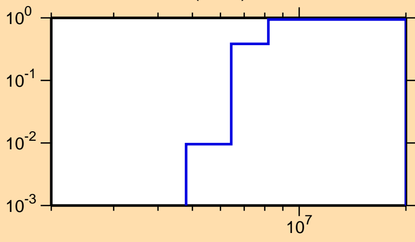
\sigma vs. E for ^{40}\text{Cl}(n,2n)
