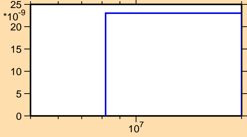
\sigma vs. E for ^{40}\text{Cl}(n,2np)
