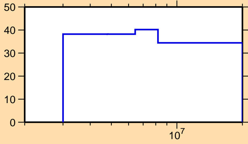
\Delta\sigma/\sigma vs. E for ^{40}\text{Cl}(n,p)
