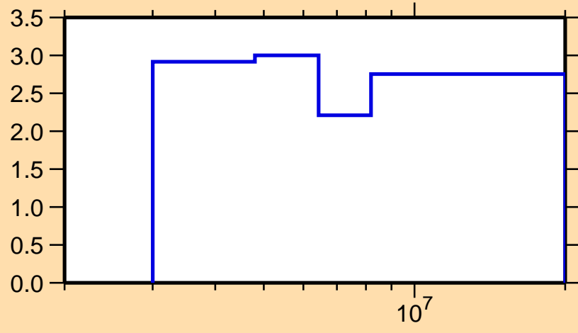
\Delta\sigma/\sigma vs. E for ^{40}\text{Cl}(n,n\text{onel.})
