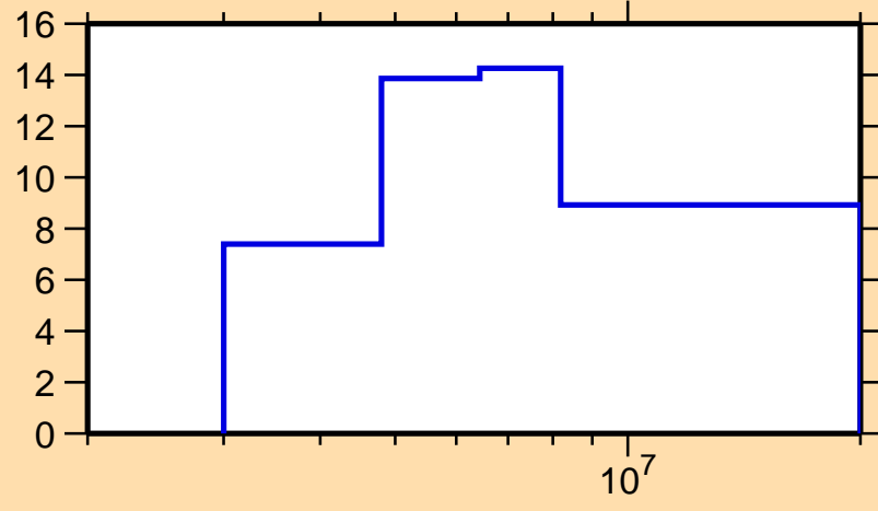
\Delta\sigma/\sigma vs. E for ^{40}\text{Cl}(n,n_1)
