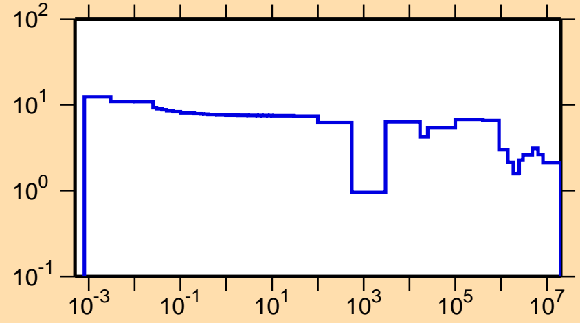
\Delta\sigma/\sigma vs. E for ^{40}\text{Cl}(n,\text{tot.})
