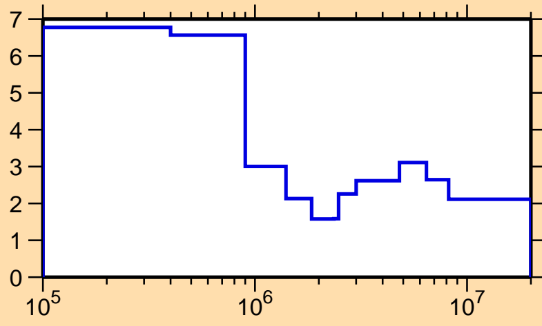
\Delta\sigma/\sigma vs. E for ^{40}\text{Cl}(n,\text{tot.})
