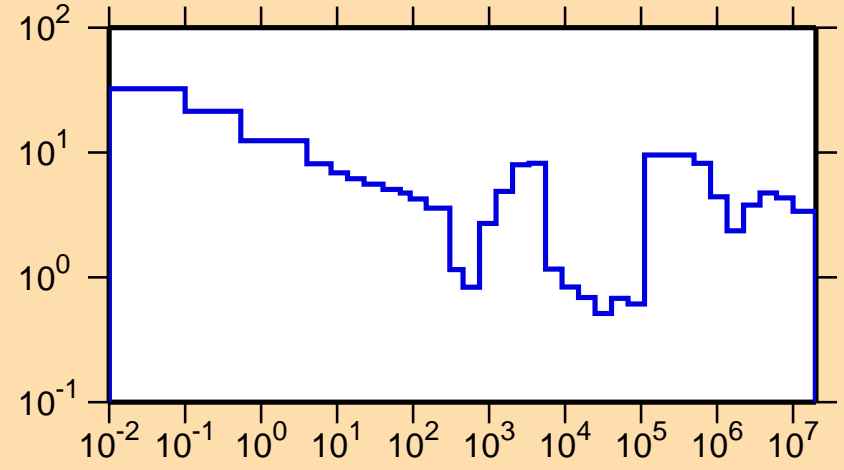
\Delta\sigma/\sigma vs. E for ^{41}\text{Cl}(n,\text{tot.})
