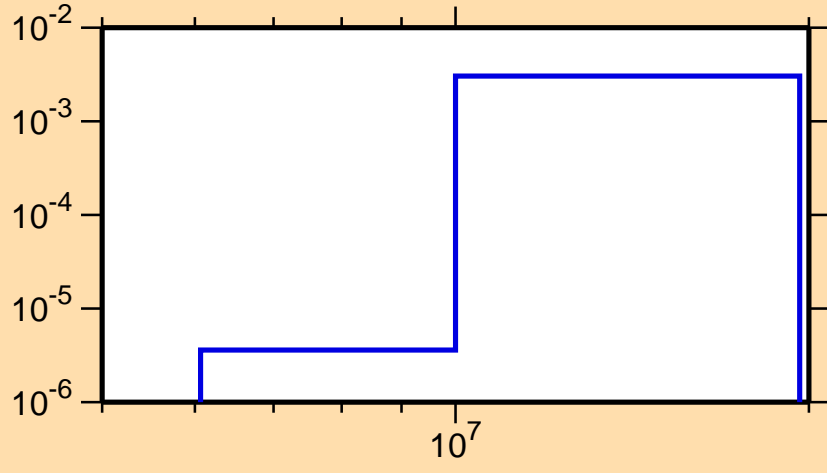
\sigma vs. E for ^{41}\text{Cl}(n,p)
