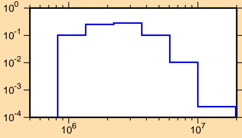
\sigma vs. E for ^{41}\text{Cl}(n,n_2)
