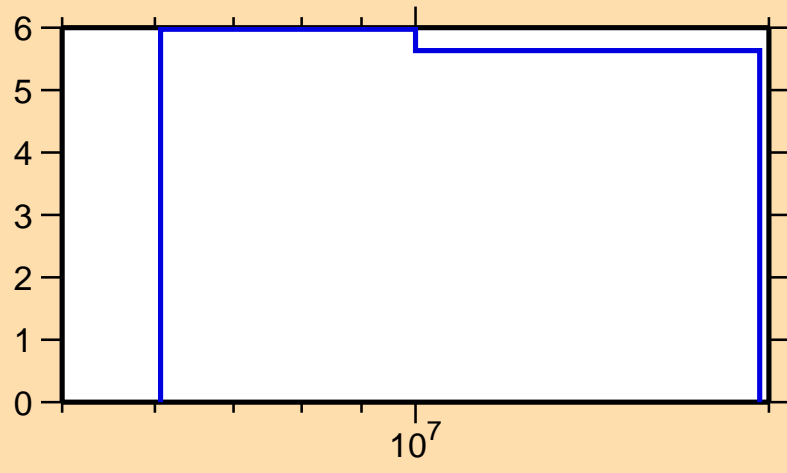
\Delta\sigma/\sigma vs. E for ^{41}\text{Cl}(n,2n)
