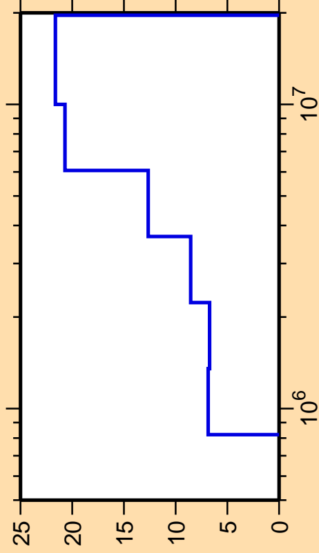
\Delta\sigma/\sigma vs. E for ^{41}\text{Cl}(n,n_2)
