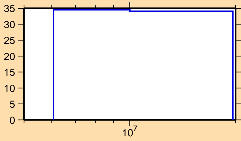
\Delta\sigma/\sigma vs. E for ^{41}\text{Cl}(n,p)
