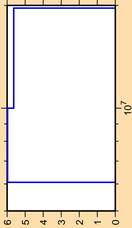
\Delta\sigma/\sigma vs. E for ^{41}\text{Cl}(n,2n)
