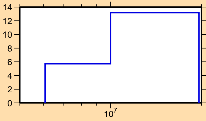
\Delta\sigma/\sigma vs. E for ^{41}\text{Cl}(n,ncont.)
