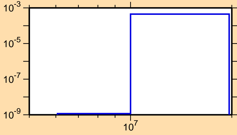
\sigma vs. E for ^{41}\text{Cl}(n,\alpha)
