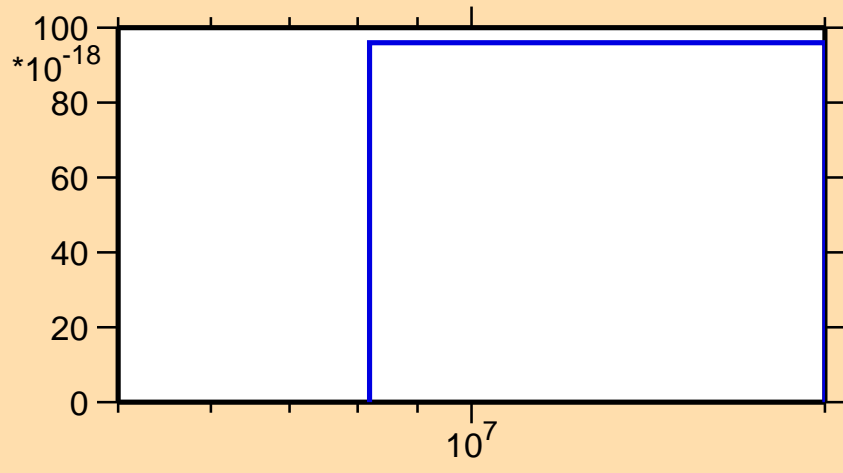
\sigma vs. E for ^{41}\text{Cl}(n,2np)
