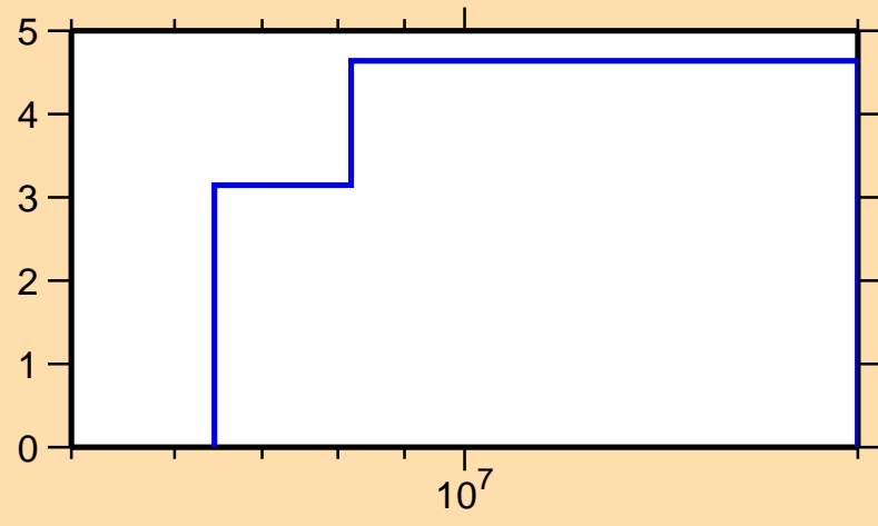
\Delta\sigma/\sigma vs. E for ^{41}\text{Cl}(n,\text{inel.})
