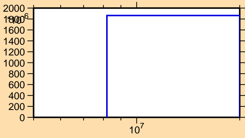
\sigma vs. E for ^{41}\text{Cl}(n,d)
