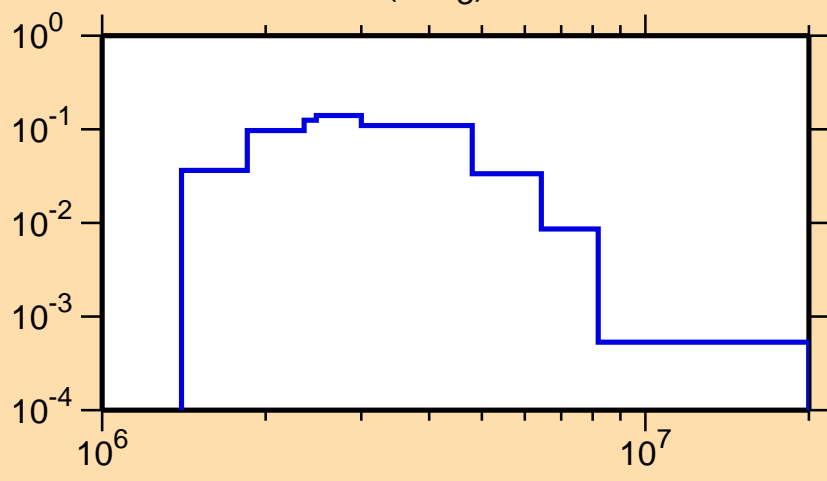
\sigma vs. E for ^{41}\text{Cl}(n,n_3)
