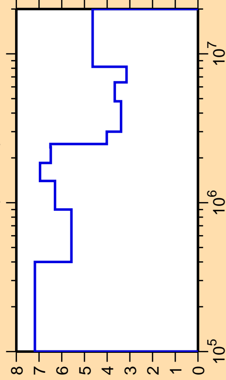
\Delta\sigma/\sigma vs. E for ^{41}\text{Cl}(n,\text{inel.})
