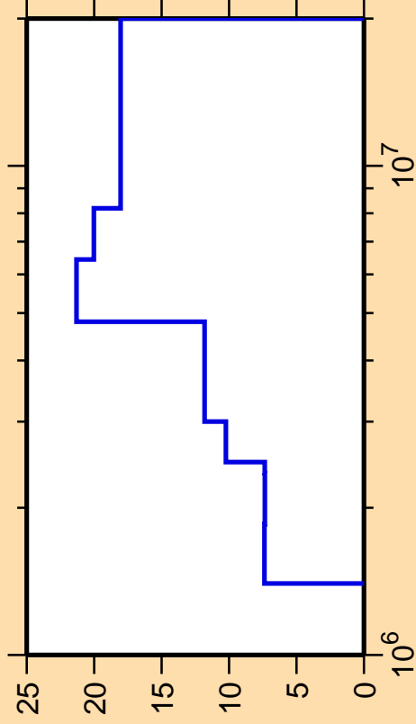
\Delta\sigma/\sigma vs. E for ^{41}\text{Cl}(n,n_3)
