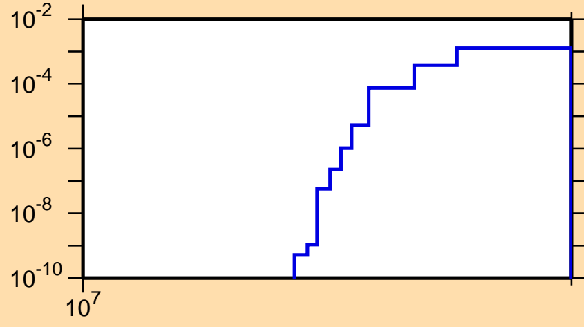
\sigma vs. E for ^{42}\text{Cl}(n,np)
