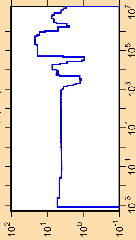
\Delta\sigma/\sigma vs. E for ^{42}\text{Cl}(n,\text{tot.})
