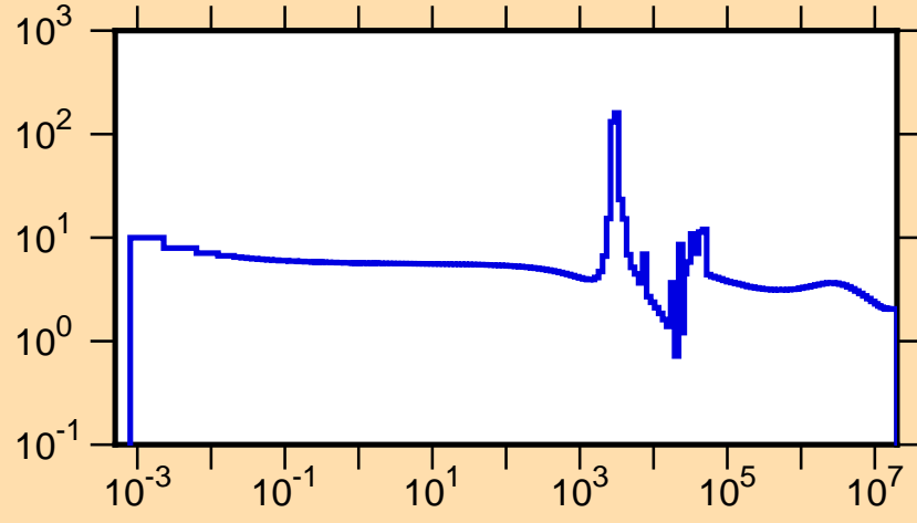
\sigma vs. E for ^{42}\text{Cl}(n,\text{tot.})
