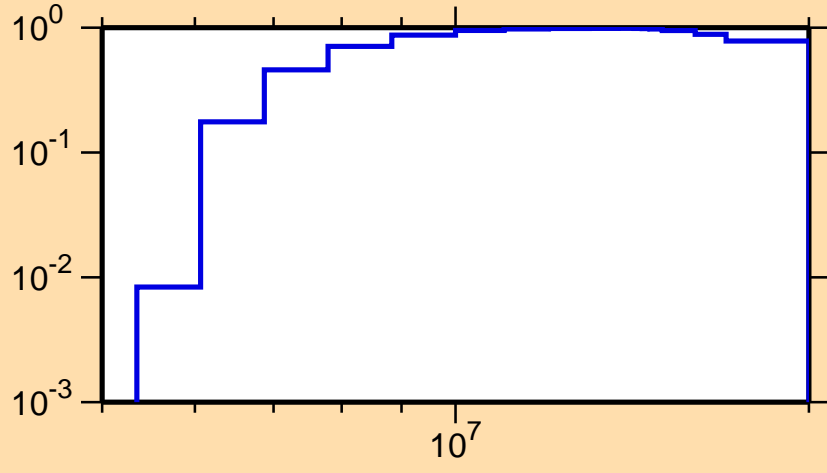
\sigma vs. E for ^{42}\text{Cl}(n,2n)
