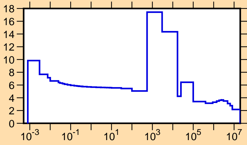
\sigma vs. E for ^{42}\text{Cl}(n,\text{tot.})
