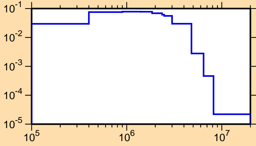
\sigma vs. E for ^{42}\text{Cl}(n,n_1)
