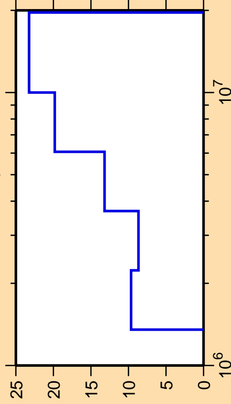
\Delta\sigma/\sigma vs. E for ^{43}\text{Cl}(n,n_3)
