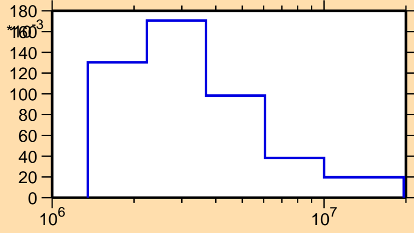
\sigma vs. E for ^{43}\text{Cl}(n,n_3)
