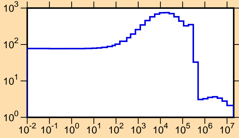
\sigma vs. E for ^{43}\text{Cl}(n,\text{tot.})
