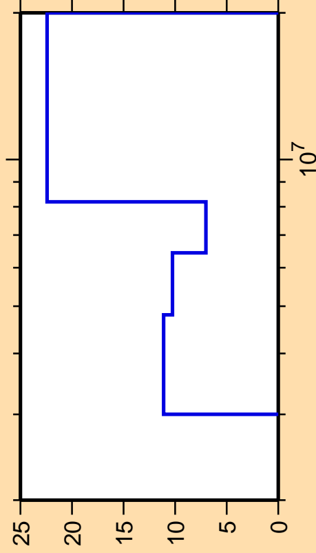
\Delta\sigma/\sigma vs. E for ^{43}\text{Cl}(n,\text{ncont.})
