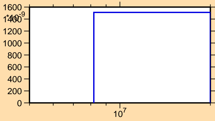
\sigma vs. E for ^{43}\text{Cl}(n,np)
