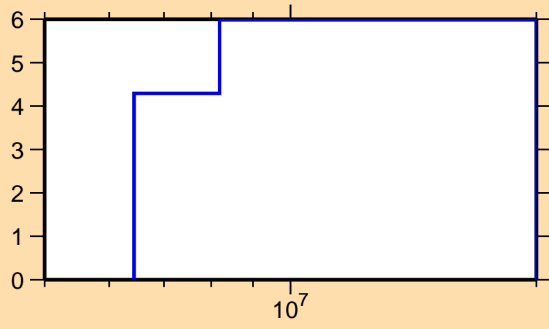
\Delta\sigma/\sigma vs. E for ^{43}\text{Cl}(n,\text{nonel.})
