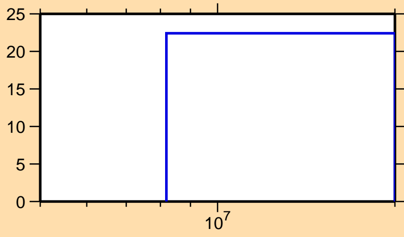
\Delta\sigma/\sigma vs. E for ^{43}\text{Cl}(n,ncont.)
