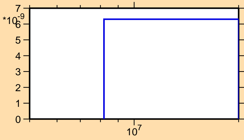
\sigma vs. E for ^{43}\text{Cl}(n,nt)
