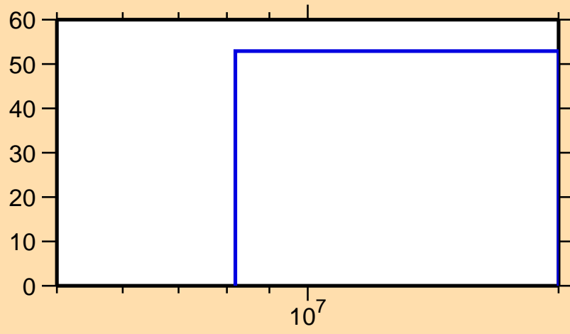
\Delta\sigma/\sigma vs. E for ^{43}\text{Cl}(n,p)
