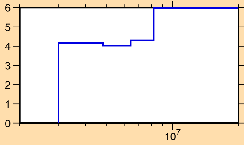
\Delta\sigma/\sigma vs. E for ^{43}\text{Cl}(n,n\text{onel.})
