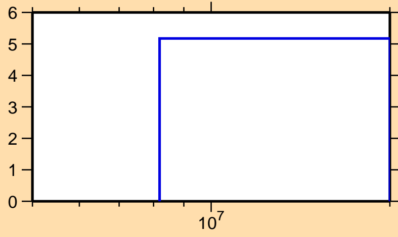
\Delta\sigma/\sigma vs. E for ^{43}\text{Cl}(n,\text{el.})
