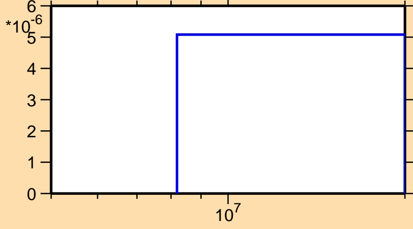
\sigma vs. E for ^{43}\text{Cl}(n,t)
