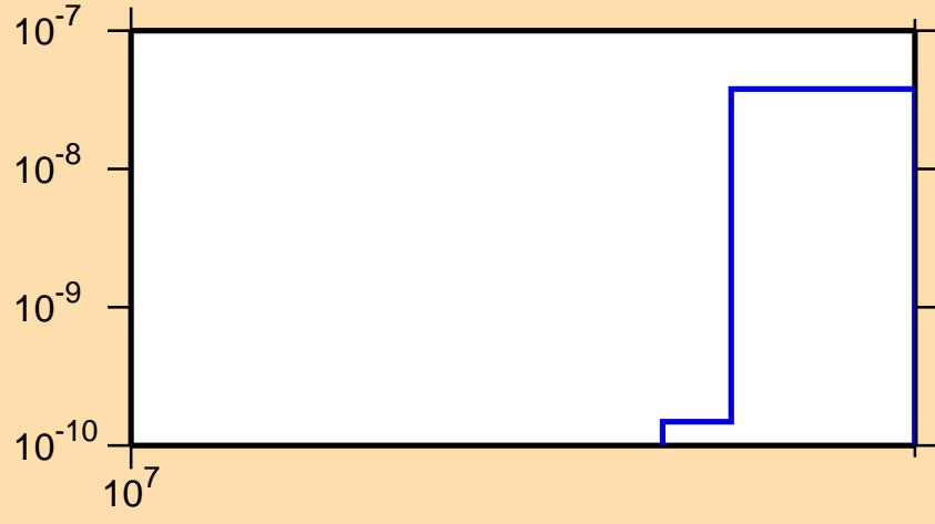
\sigma vs. E for ^{232}\text{Cm}(n,nt)
