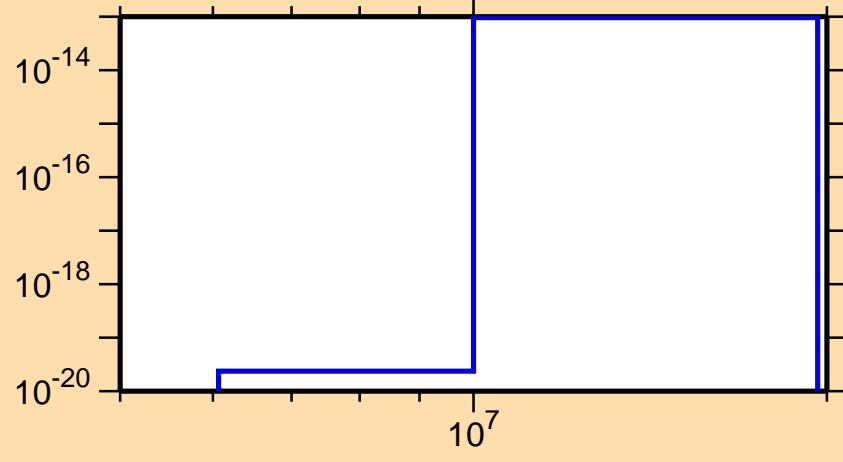
\sigma vs. E for ^{232}\text{Cm}(n,2n\alpha)
