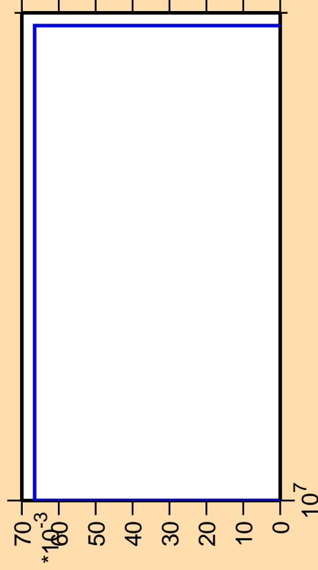
\Delta\sigma/\sigma vs. E for ^{232}\text{Cm}(n,2np)
