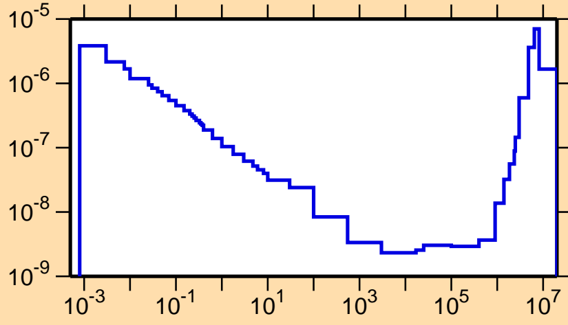
\sigma vs. E for ^{232}\text{Cm}(n,p)
