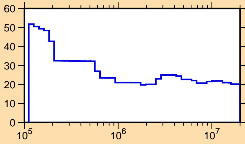
\Delta\sigma/\sigma vs. E for ^{233}\text{Cm}(n,\text{nonel.})
