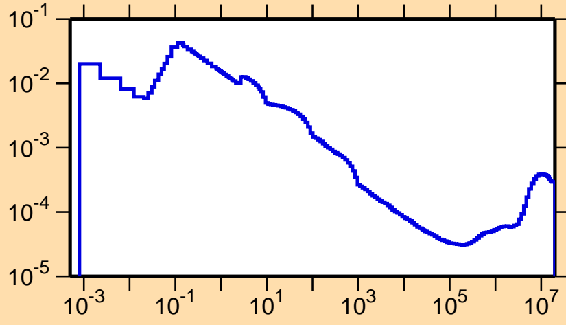
\sigma vs. E for ^{233}\text{Cm}(n,p)
