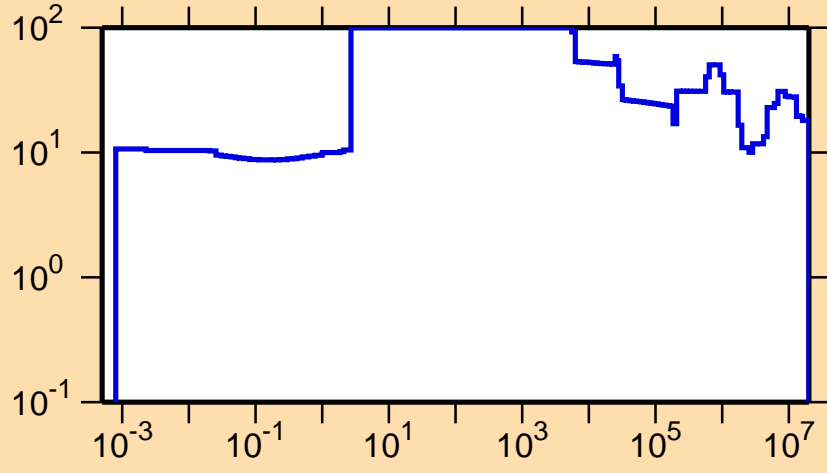
\Delta\sigma/\sigma vs. E for ^{233}\text{Cm}(n,tot.)
