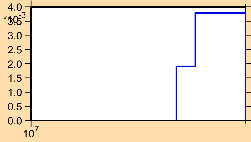
\sigma vs. E for ^{233}\text{Cm}(n,2np)
