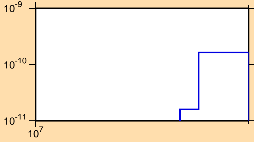
\sigma vs. E for ^{233}\text{Cm} (mt 45)
