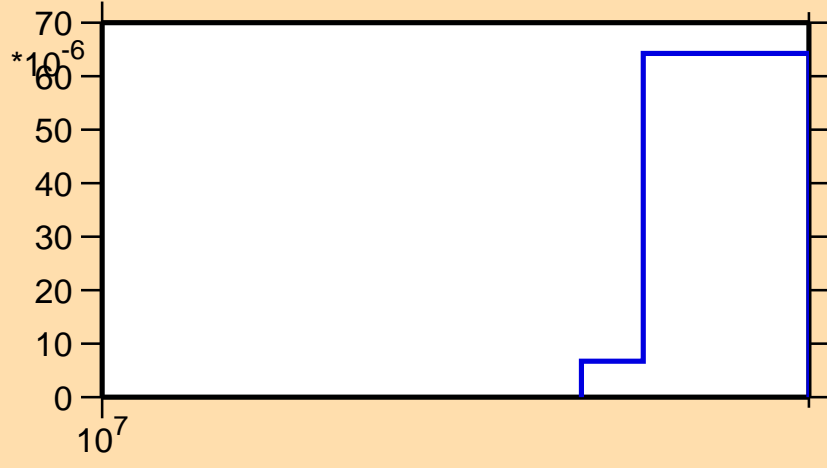
\sigma vs. E for ^{233}\text{Cm}(n,nd)
