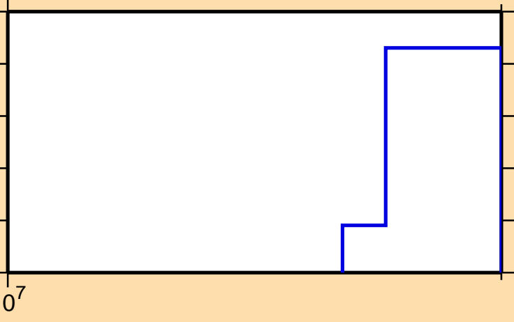
\sigma vs. E for ^{233}\text{Cm}(n,3n)
