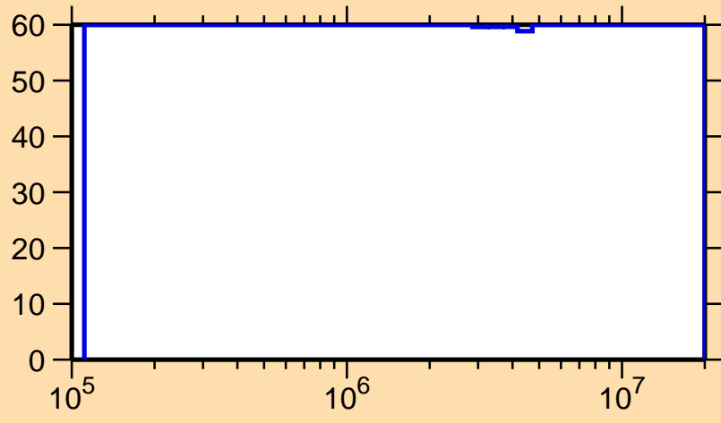
\Delta\sigma/\sigma vs. E for ^{233}\text{Cm}(n,\text{inel.})
