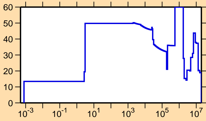
\Delta\sigma/\sigma vs. E for ^{233}\text{Cm}(n,el.)
