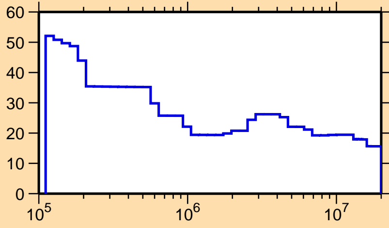
\Delta\sigma/\sigma vs. E for ^{233}\text{Cm}(n,f)
