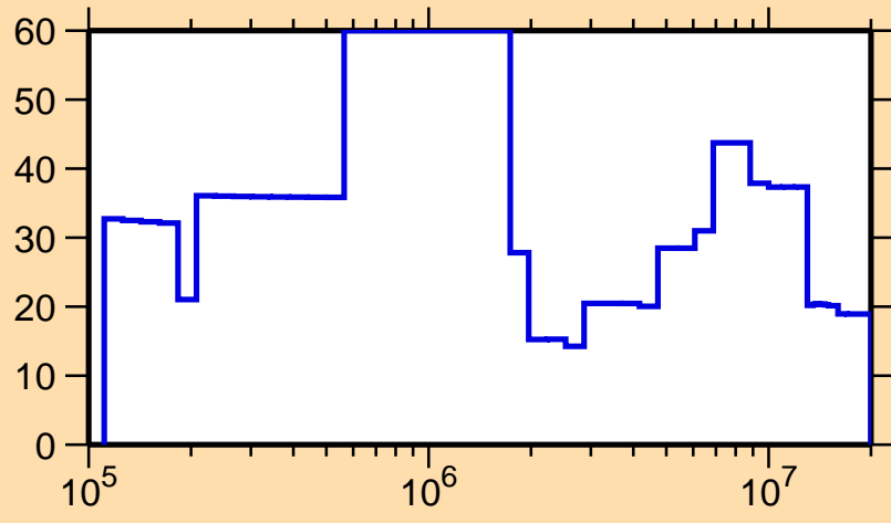
\Delta\sigma/\sigma vs. E for ^{233}\text{Cm}(n,\text{el.})
