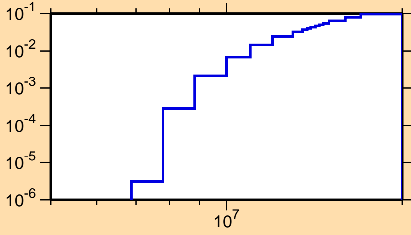
\sigma vs. E for ^{233}\text{Cm}(n,2n)
