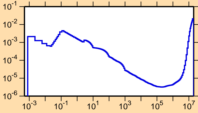
\sigma vs. E for ^{233}\text{Cm}(n,\alpha)
