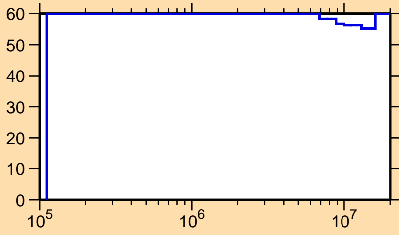
\Delta\sigma/\sigma vs. E for ^{233}\text{Cm}(n,n_1)
