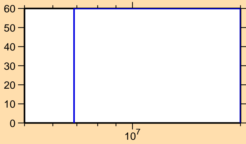
\Delta\sigma/\sigma vs. E for ^{233}\text{Cm}(n,2n)
