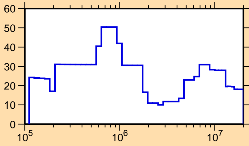
\Delta\sigma/\sigma vs. E for ^{233}\text{Cm}(n,\text{tot.})
