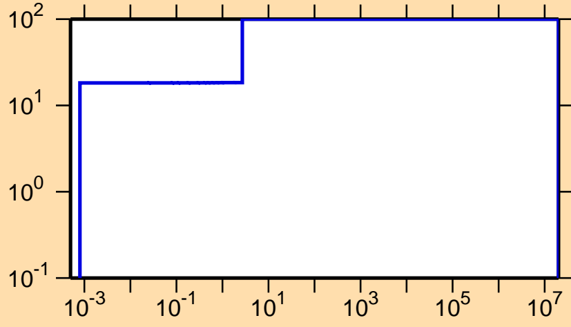
\Delta\sigma/\sigma vs. E for ^{233}\text{Cm}(n,\gamma)
