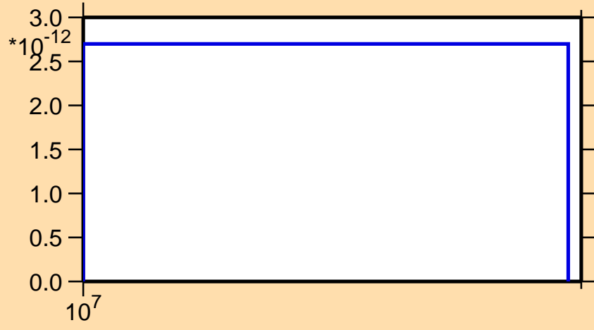
\sigma vs. E for ^{233}\text{Cm} (mt 45)
