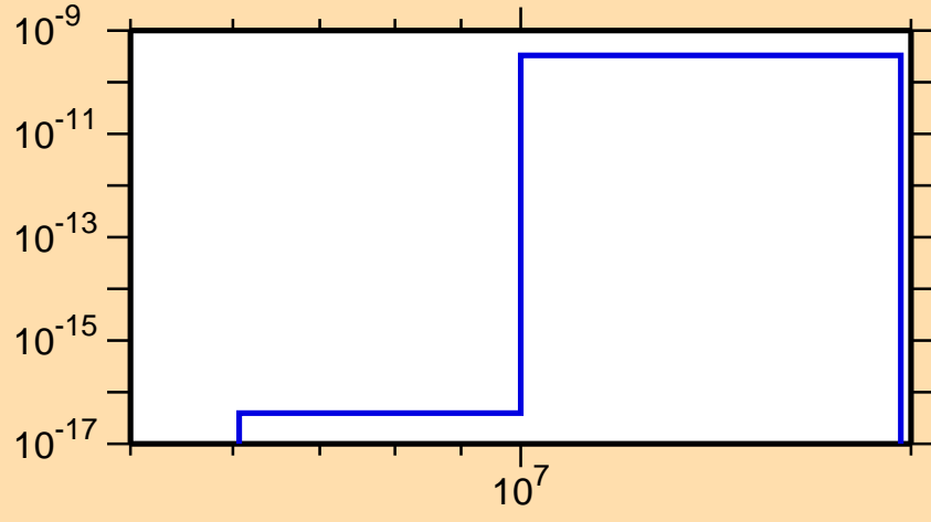
\sigma vs. E for ^{233}\text{Cm}(n,\text{He3})
