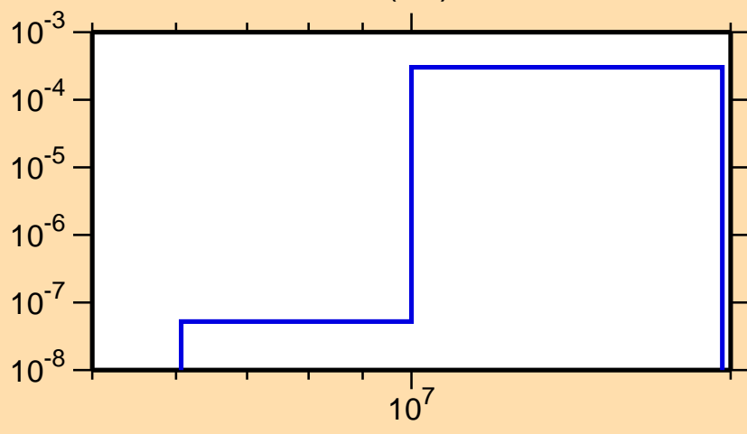
\sigma vs. E for ^{233}\text{Cm}(n,t)
